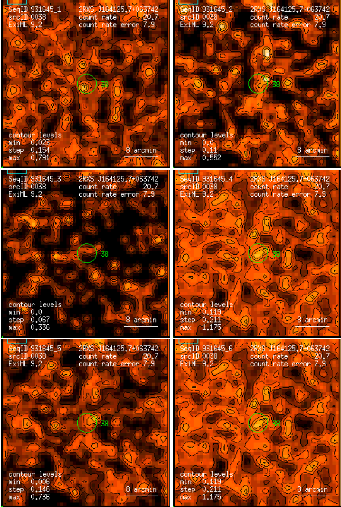
Figure 38: RASS 931645: detection 0038: band rate images, Gaussian filter: (1) PSPC channels 11 – 41, (2) 52 – 90, (3) 91 – 201, (4) 11 – 235, (5) 52 – 201, (6) 11 – 201. Broad band rates in counts/ks. Band rate contour levels in counts/ks/arcmin 2 .
