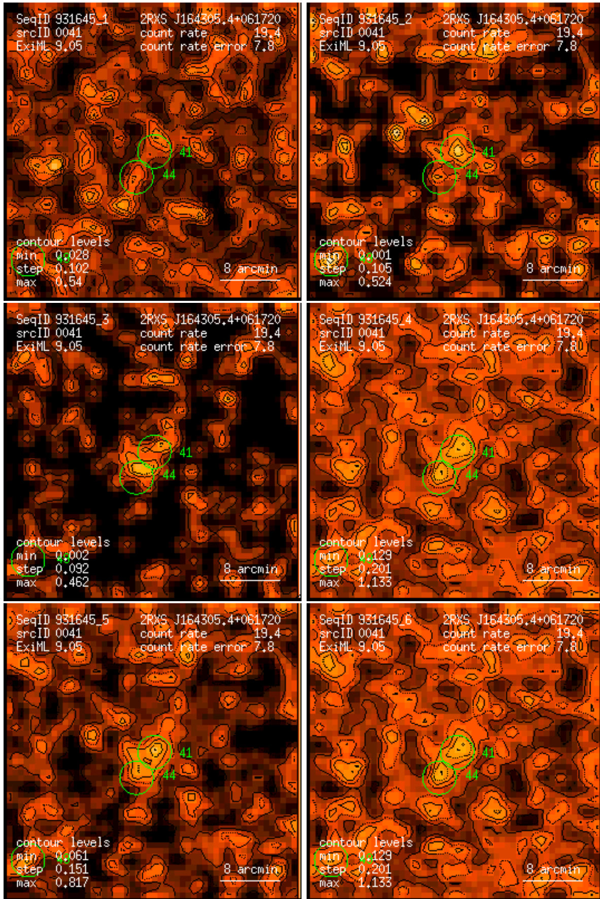
Figure 41: RASS 931645: detection 0041: band rate images, Gaussian filter: (1) PSPC channels 11 – 41, (2) 52 – 90, (3) 91 – 201, (4) 11 – 235, (5) 52 – 201, (6) 11 – 201. Broad band rates in counts/ks. Band rate contour levels in counts/ks/arcmin 2 .
