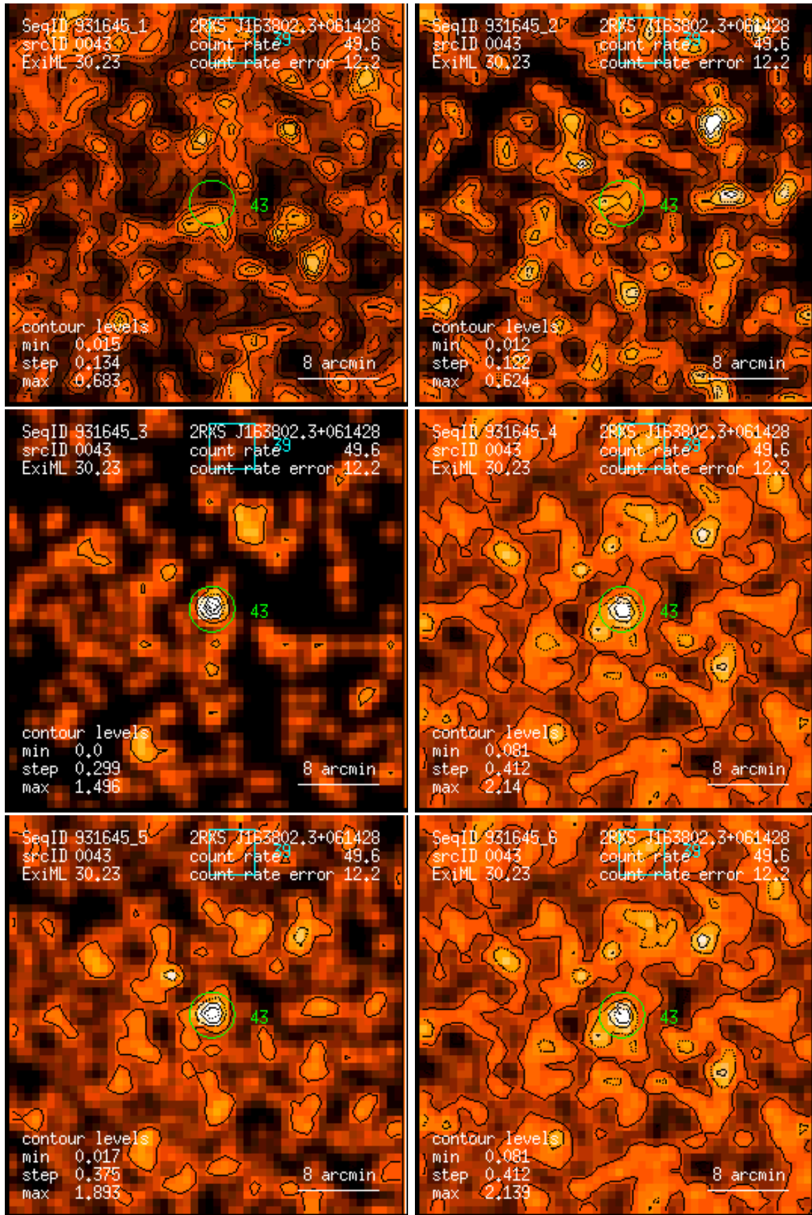
Figure 43: RASS 931645: detection 0043: band rate images, Gaussian filter: (1) PSPC channels 11 – 41, (2) 52 – 90, (3) 91 – 201, (4) 11 – 235, (5) 52 – 201, (6) 11 – 201. Broad band rates in counts/ks. Band rate contour levels in counts/ks/arcmin 2 .
