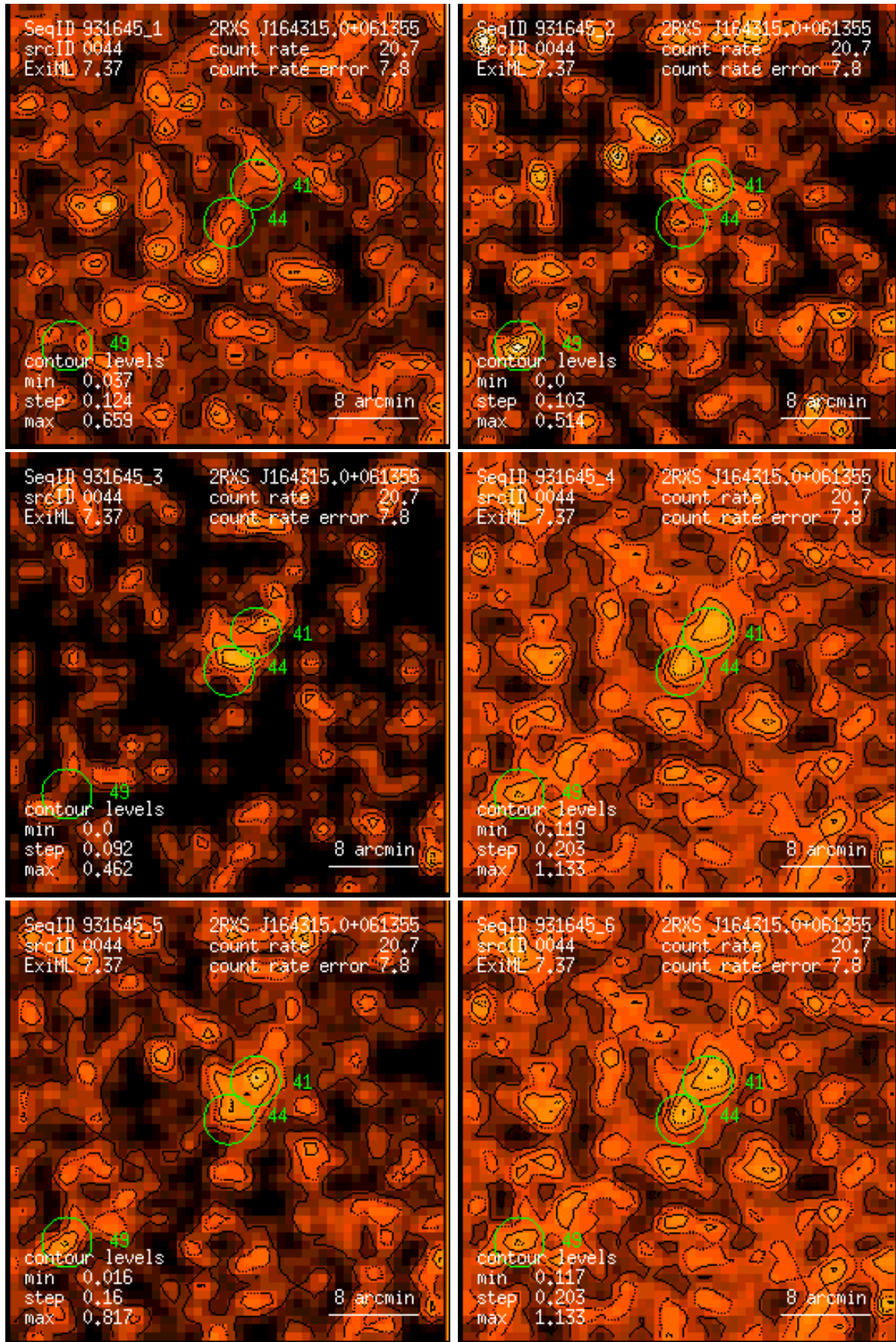
Figure 44: RASS 931645: detection 0044: band rate images, Gaussian filter: (1) PSPC channels 11 – 41, (2) 52 – 90, (3) 91 – 201, (4) 11 – 235, (5) 52 – 201, (6) 11 – 201. Broad band rates in counts/ks. Band rate contour levels in counts/ks/arcmin 2 .
