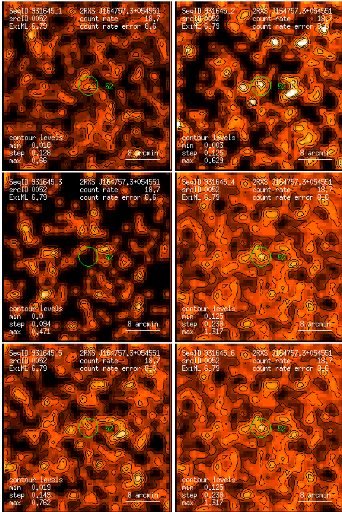
Figure 52: RASS 931645: detection 0052: band rate images, Gaussian filter: (1) PSPC channels 11 – 41, (2) 52 – 90, (3) 91 – 201, (4) 11 – 235, (5) 52 – 201, (6) 11 – 201. Broad band rates in counts/ks. Band rate contour levels in counts/ks/arcmin 2 .
