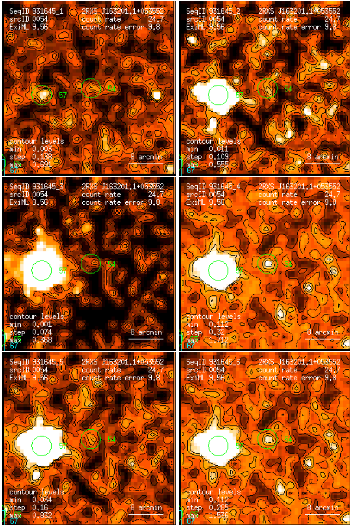
Figure 54: RASS 931645: detection 0054: band rate images, Gaussian filter: (1) PSPC channels 11 – 41, (2) 52 – 90, (3) 91 – 201, (4) 11 – 235, (5) 52 – 201, (6) 11 – 201. Broad band rates in counts/ks. Band rate contour levels in counts/ks/arcmin 2 .
