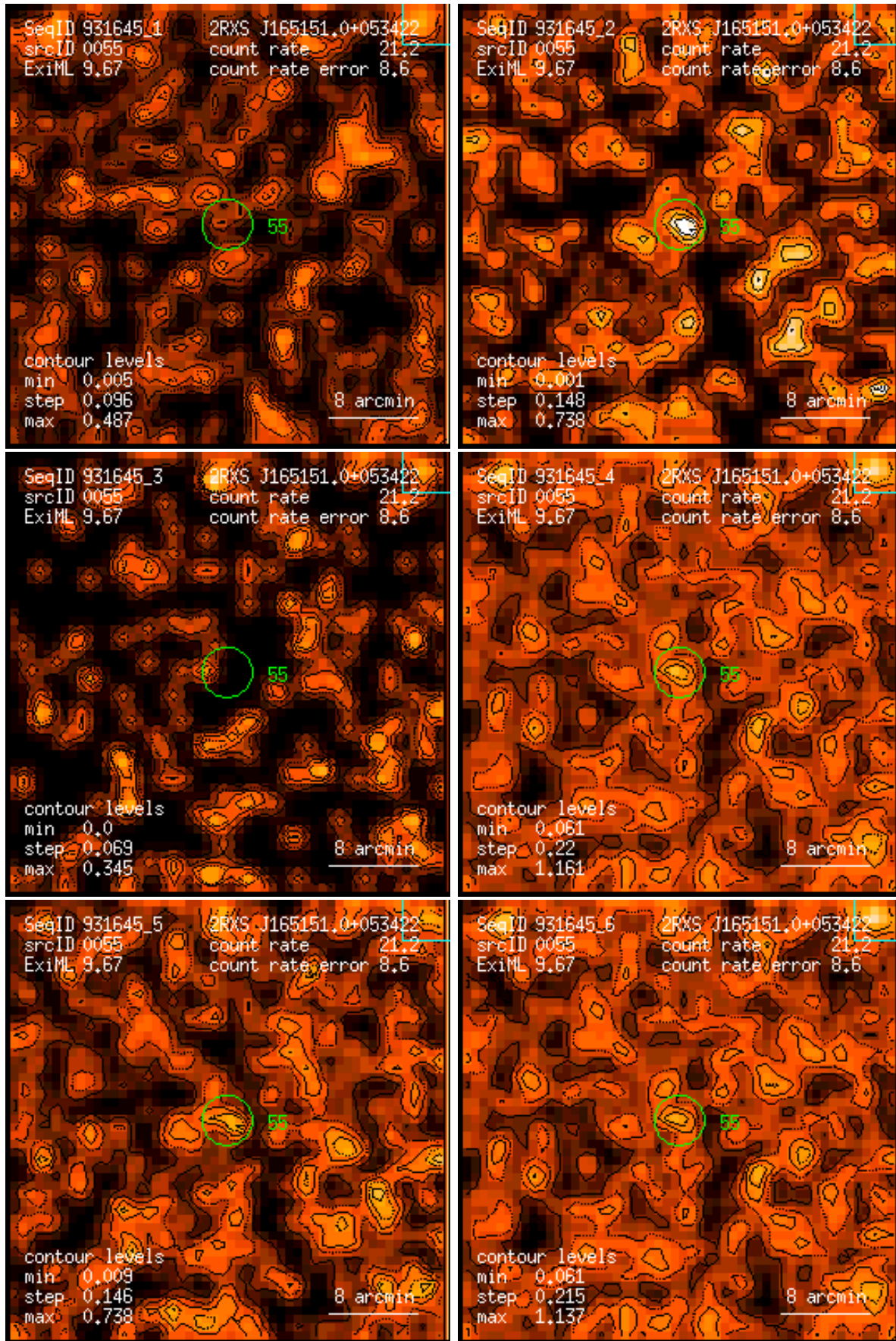
Figure 55: RASS 931645: detection 0055: band rate images, Gaussian filter: (1) PSPC channels 11 – 41, (2) 52 – 90, (3) 91 – 201, (4) 11 – 235, (5) 52 – 201, (6) 11 – 201. Broad band rates in counts/ks. Band rate contour levels in counts/ks/arcmin 2 .
