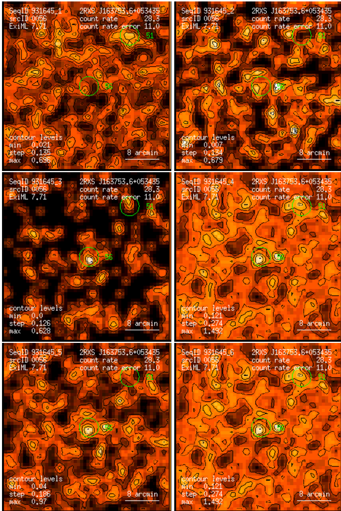
Figure 56: RASS 931645: detection 0056: band rate images, Gaussian filter: (1) PSPC channels 11 – 41, (2) 52 – 90, (3) 91 – 201, (4) 11 – 235, (5) 52 – 201, (6) 11 – 201. Broad band rates in counts/ks. Band rate contour levels in counts/ks/arcmin 2 .
