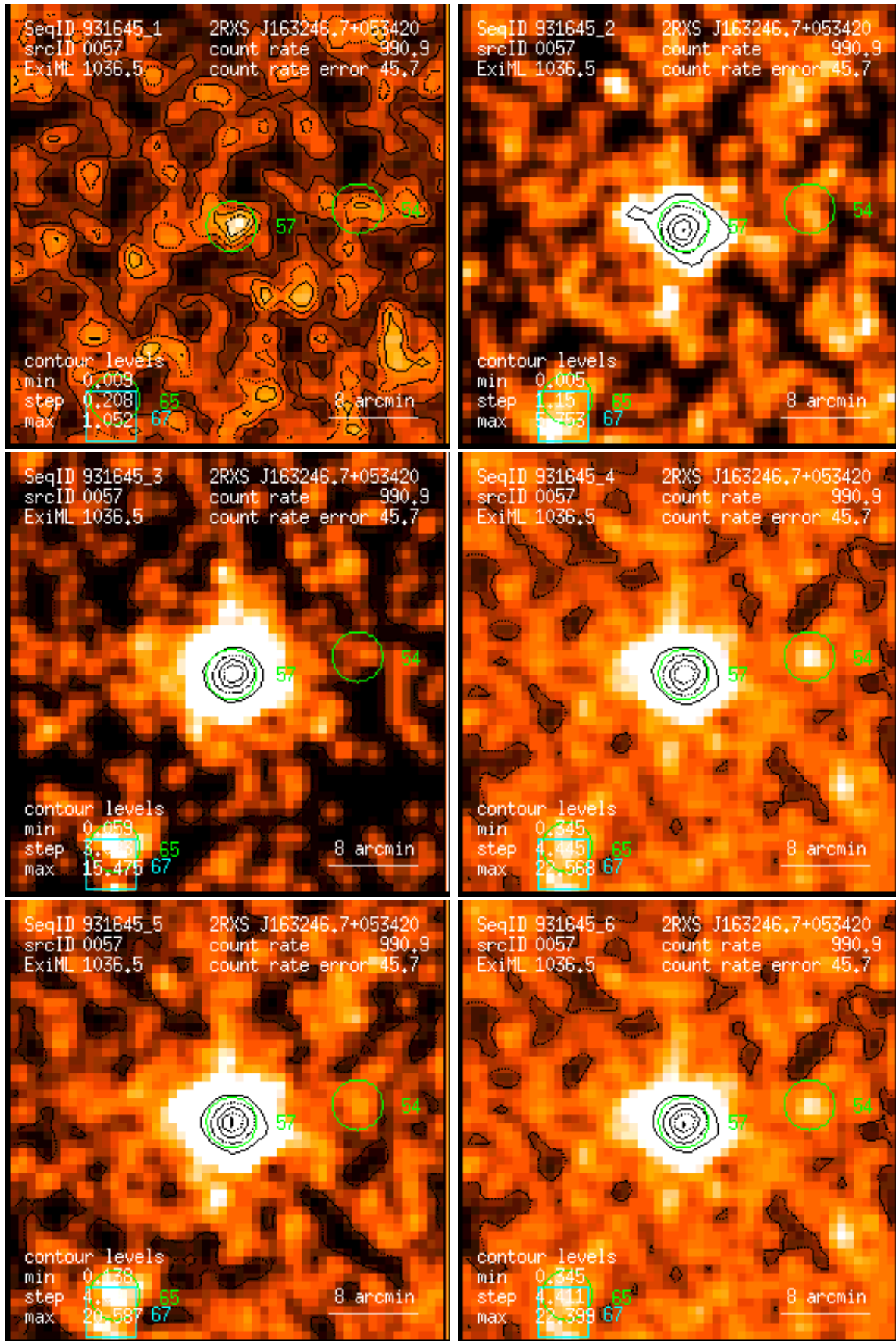
Figure 57: RASS 931645: detection 0057: band rate images, Gaussian filter: (1) PSPC channels 11 – 41, (2) 52 – 90, (3) 91 – 201, (4) 11 – 235, (5) 52 – 201, (6) 11 – 201. Broad band rates in counts/ks. Band rate contour levels in counts/ks/arcmin 2 .
