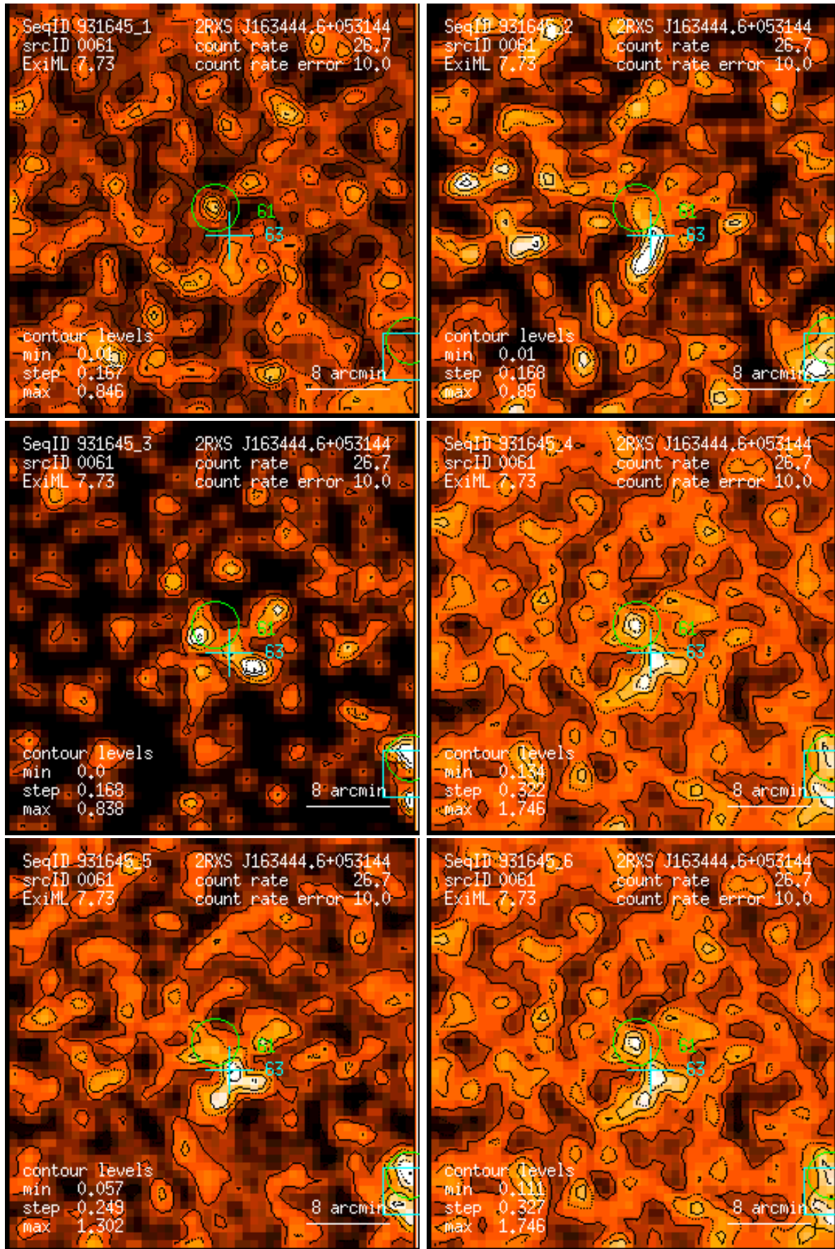
Figure 61: RASS 931645: detection 0061: band rate images, Gaussian filter: (1) PSPC channels 11 – 41, (2) 52 – 90, (3) 91 – 201, (4) 11 – 235, (5) 52 – 201, (6) 11 – 201. Broad band rates in counts/ks. Band rate contour levels in counts/ks/arcmin 2 .
