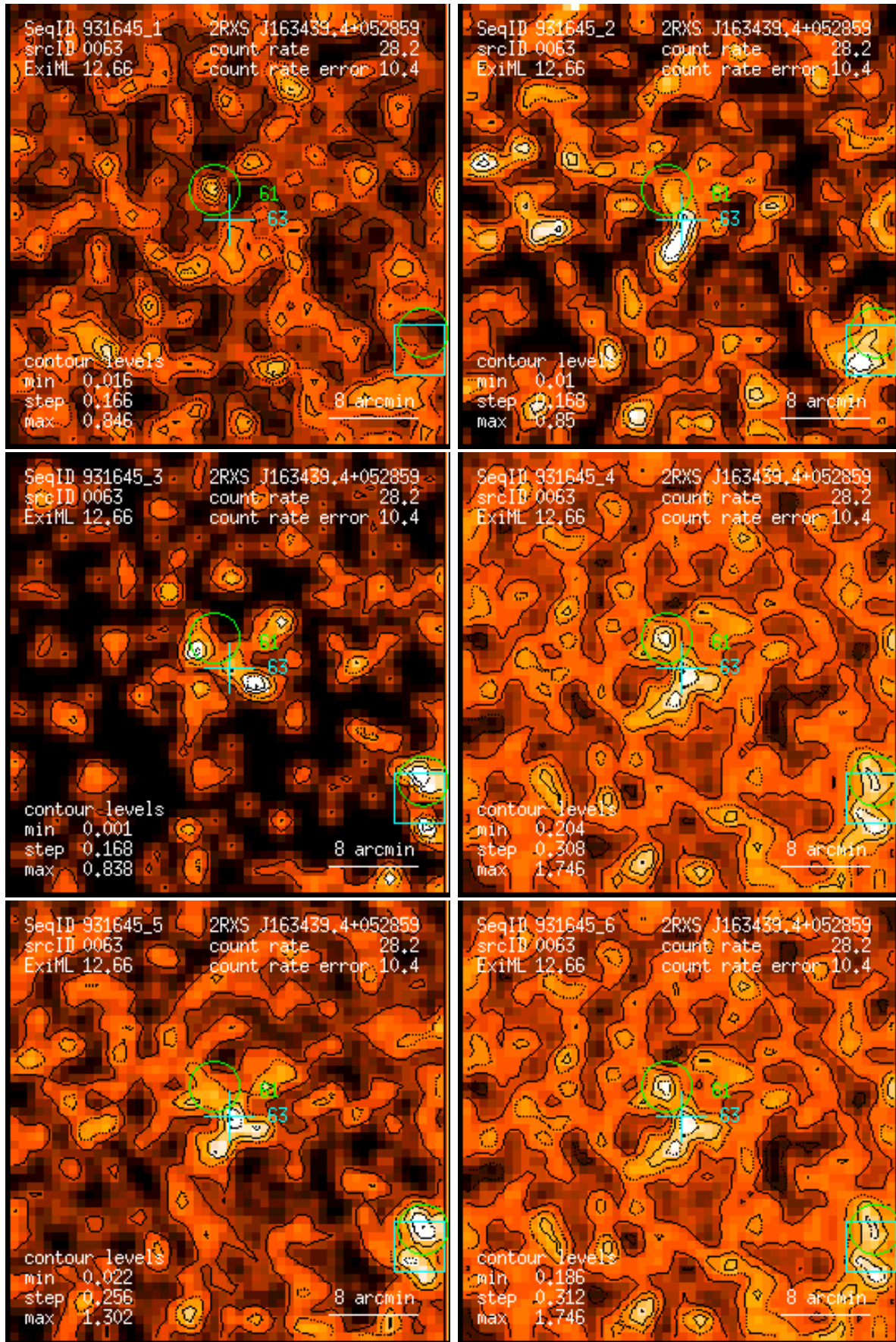
Figure 63: RASS 931645: detection 0063: band rate images, Gaussian filter: (1) PSPC channels 11 – 41, (2) 52 – 90, (3) 91 – 201, (4) 11 – 235, (5) 52 – 201, (6) 11 – 201. Broad band rates in counts/ks. Band rate contour levels in counts/ks/arcmin 2 .
