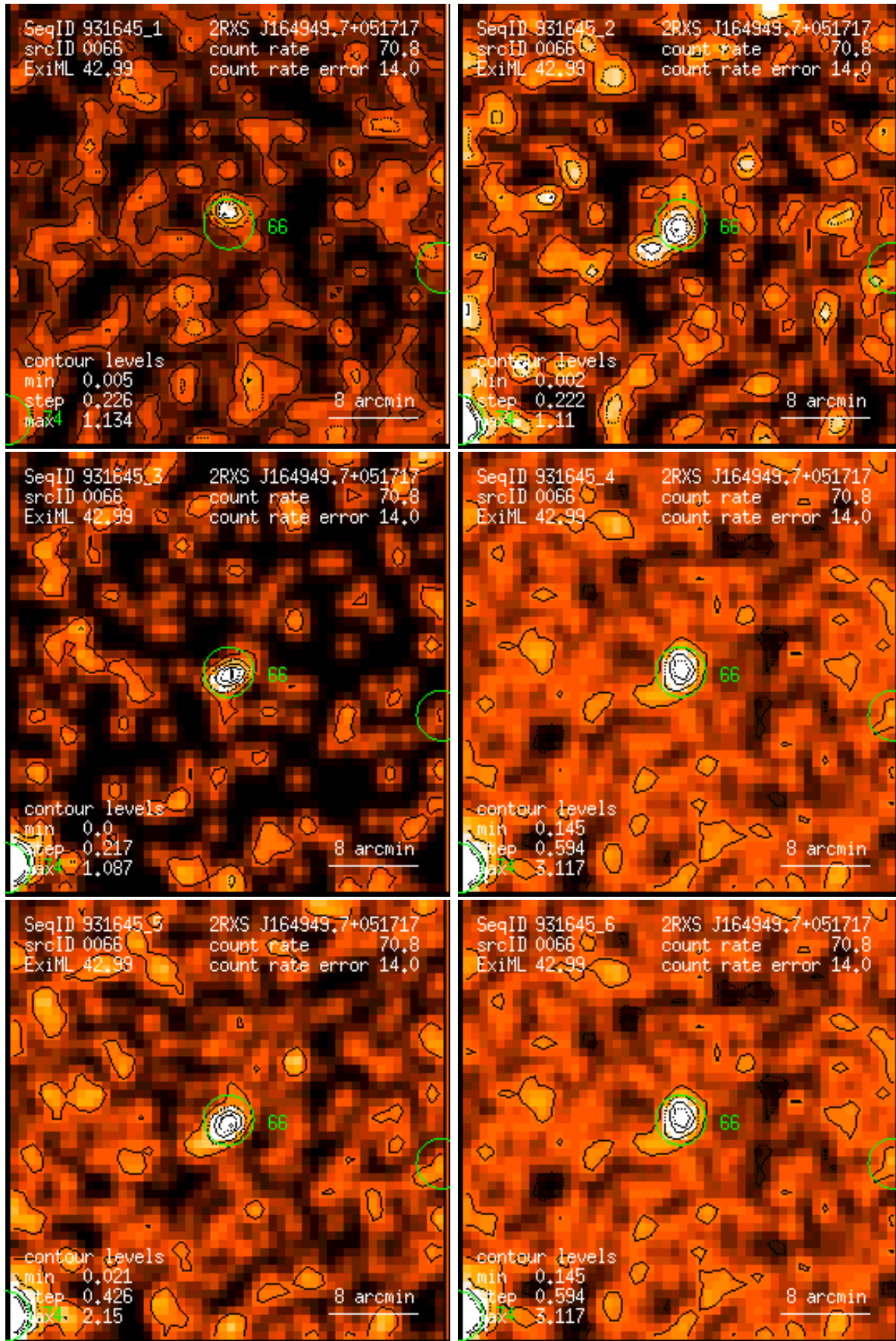
Figure 66: RASS 931645: detection 0066: band rate images, Gaussian filter: (1) PSPC channels 11 – 41, (2) 52 – 90, (3) 91 – 201, (4) 11 – 235, (5) 52 – 201, (6) 11 – 201. Broad band rates in counts/ks. Band rate contour levels in counts/ks/arcmin 2 .
