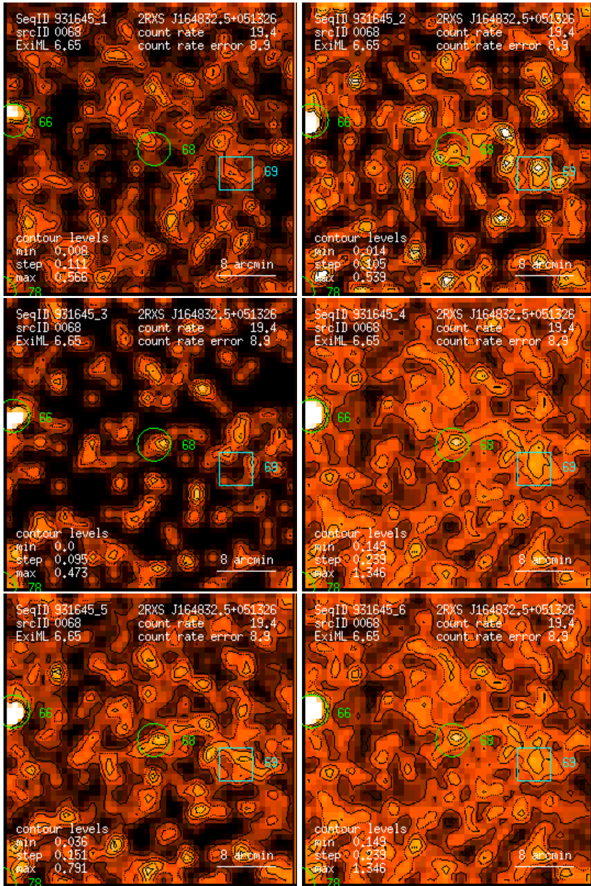
Figure 68: RASS 931645: detection 0068: band rate images, Gaussian filter: (1) PSPC channels 11 – 41, (2) 52 – 90, (3) 91 – 201, (4) 11 – 235, (5) 52 – 201, (6) 11 – 201. Broad band rates in counts/ks. Band rate contour levels in counts/ks/arcmin 2 .
