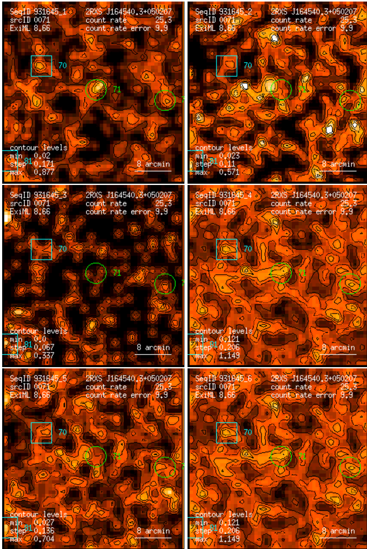
Figure 71: RASS 931645: detection 0071: band rate images, Gaussian filter: (1) PSPC channels 11 – 41, (2) 52 – 90, (3) 91 – 201, (4) 11 – 235, (5) 52 – 201, (6) 11 – 201. Broad band rates in counts/ks. Band rate contour levels in counts/ks/arcmin 2 .
