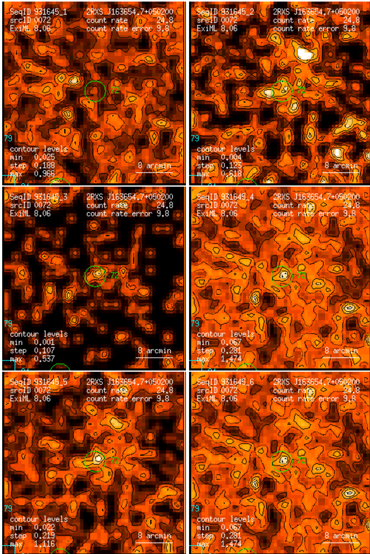
Figure 72: RASS 931645: detection 0072: band rate images, Gaussian filter: (1) PSPC channels 11 – 41, (2) 52 – 90, (3) 91 – 201, (4) 11 – 235, (5) 52 – 201, (6) 11 – 201. Broad band rates in counts/ks. Band rate contour levels in counts/ks/arcmin 2 .
