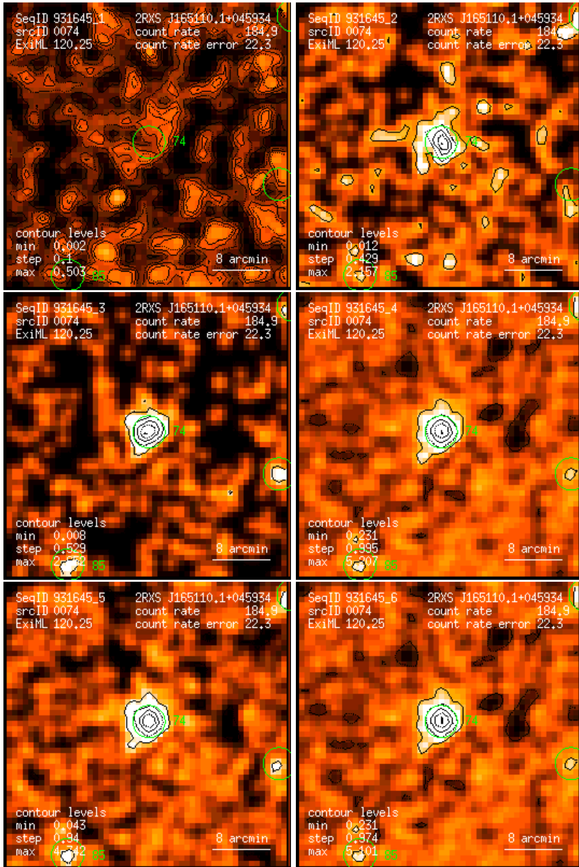
Figure 74: RASS 931645: detection 0074: band rate images, Gaussian filter: (1) PSPC channels 11 – 41, (2) 52 – 90, (3) 91 – 201, (4) 11 – 235, (5) 52 – 201, (6) 11 – 201. Broad band rates in counts/ks. Band rate contour levels in counts/ks/arcmin 2 .
