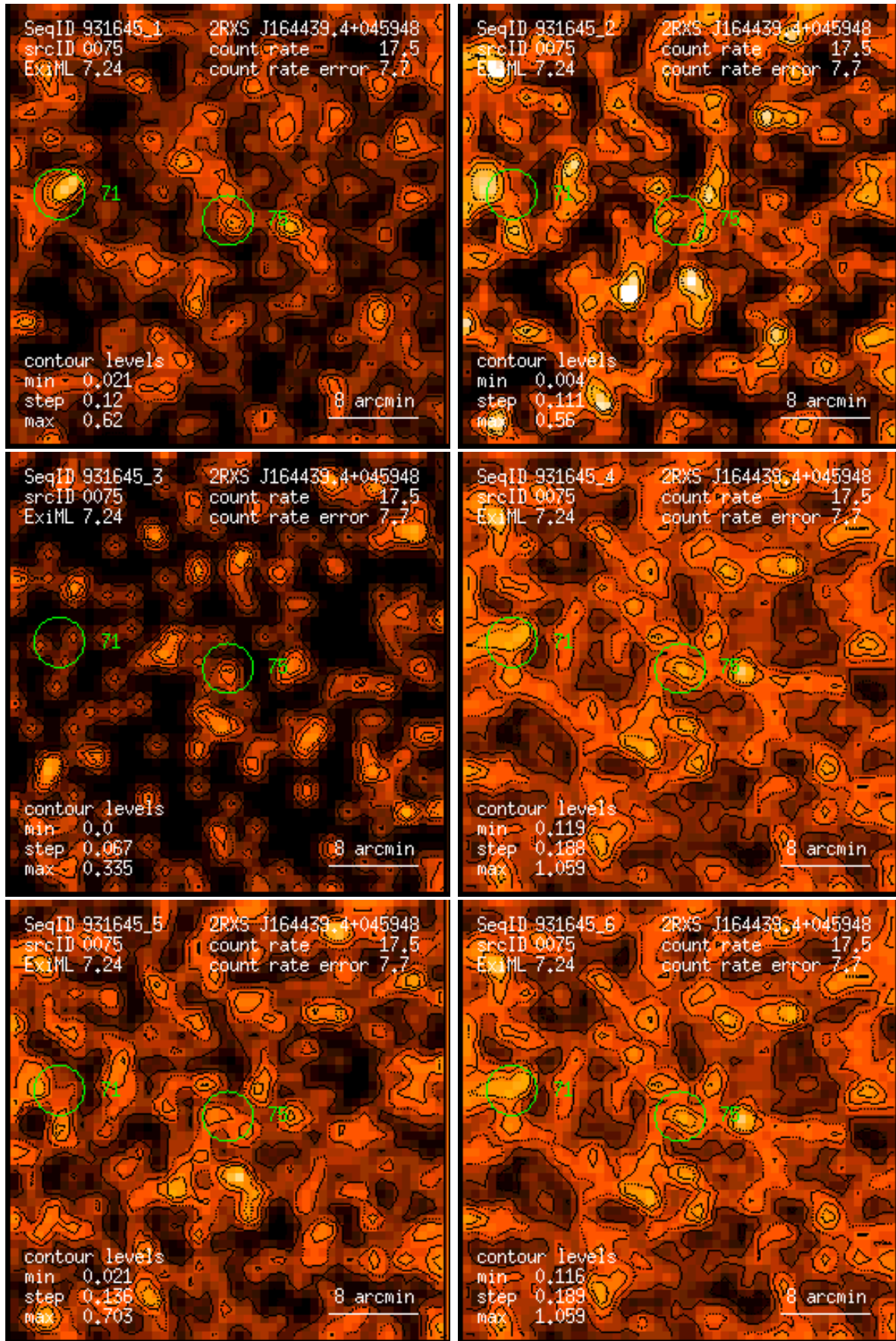
Figure 75: RASS 931645: detection 0075: band rate images, Gaussian filter: (1) PSPC channels 11 – 41, (2) 52 – 90, (3) 91 – 201, (4) 11 – 235, (5) 52 – 201, (6) 11 – 201. Broad band rates in counts/ks. Band rate contour levels in counts/ks/arcmin 2 .
