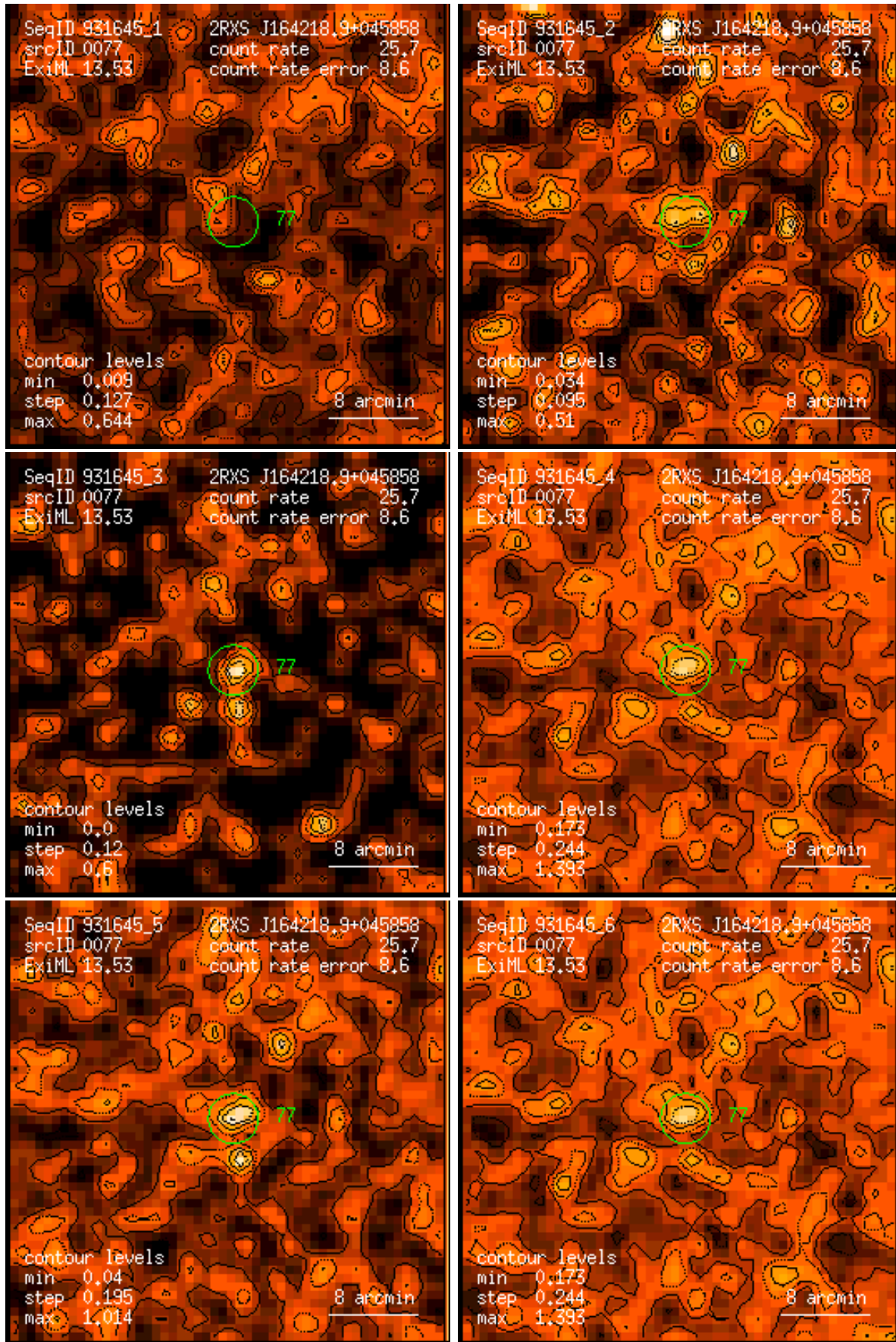
Figure 77: RASS 931645: detection 0077: band rate images, Gaussian filter: (1) PSPC channels 11 – 41, (2) 52 – 90, (3) 91 – 201, (4) 11 – 235, (5) 52 – 201, (6) 11 – 201. Broad band rates in counts/ks. Band rate contour levels in counts/ks/arcmin 2 .
