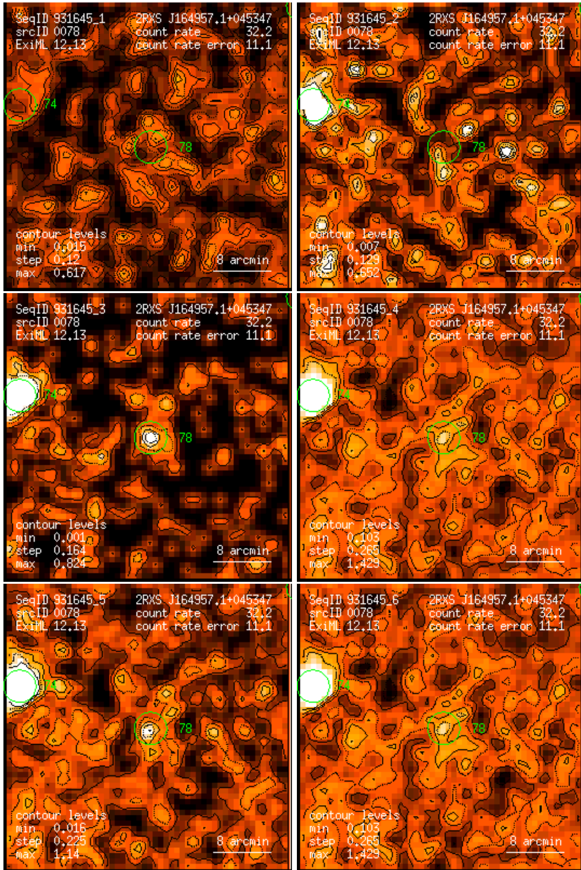
Figure 78: RASS 931645: detection 0078: band rate images, Gaussian filter: (1) PSPC channels 11 – 41, (2) 52 – 90, (3) 91 – 201, (4) 11 – 235, (5) 52 – 201, (6) 11 – 201. Broad band rates in counts/ks. Band rate contour levels in counts/ks/arcmin 2 .
