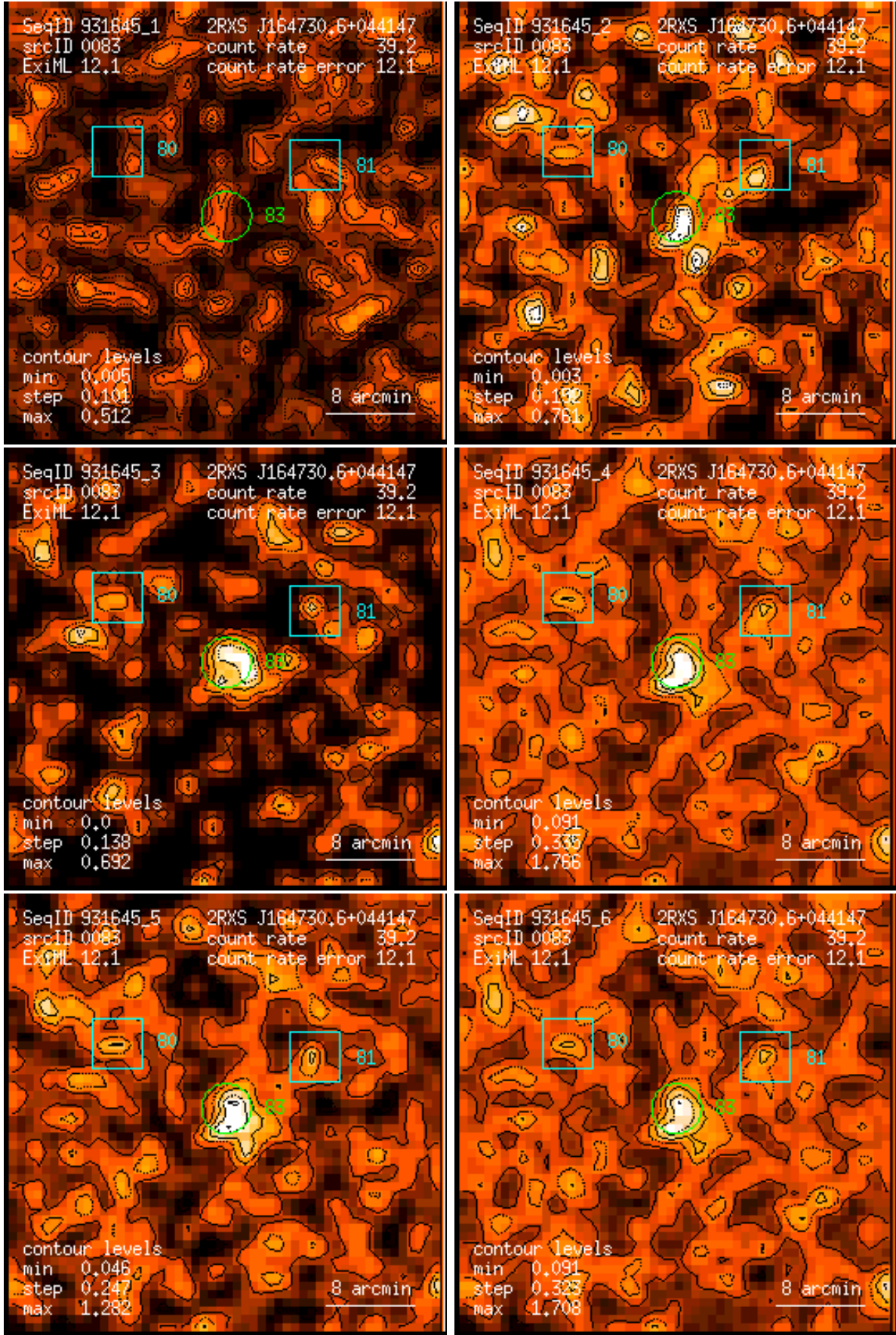
Figure 83: RASS 931645: detection 0083: band rate images, Gaussian filter: (1) PSPC channels 11 – 41, (2) 52 – 90, (3) 91 – 201, (4) 11 – 235, (5) 52 – 201, (6) 11 – 201. Broad band rates in counts/ks. Band rate contour levels in counts/ks/arcmin 2 .
