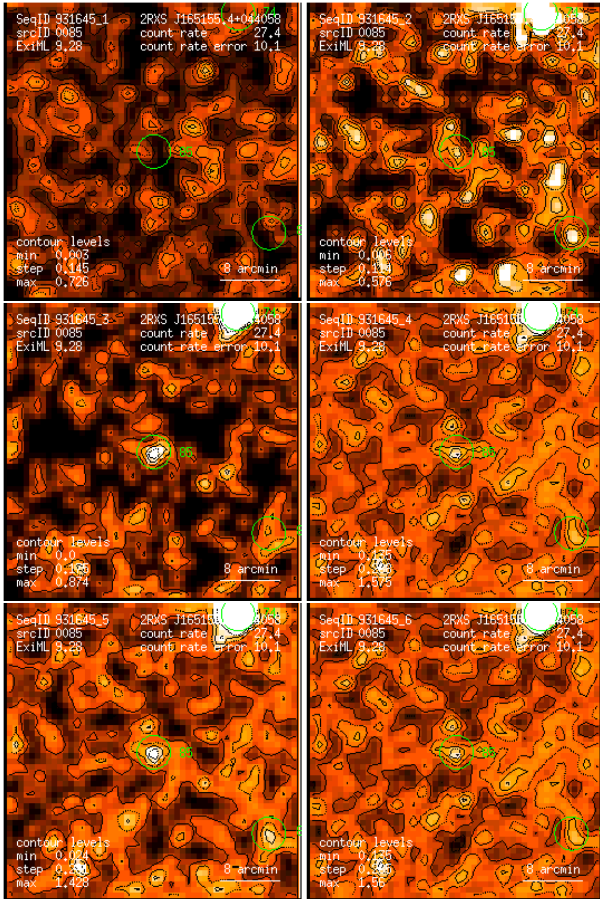
Figure 85: RASS 931645: detection 0085: band rate images, Gaussian filter: (1) PSPC channels 11 – 41, (2) 52 – 90, (3) 91 – 201, (4) 11 – 235, (5) 52 – 201, (6) 11 – 201. Broad band rates in counts/ks. Band rate contour levels in counts/ks/arcmin 2 .
