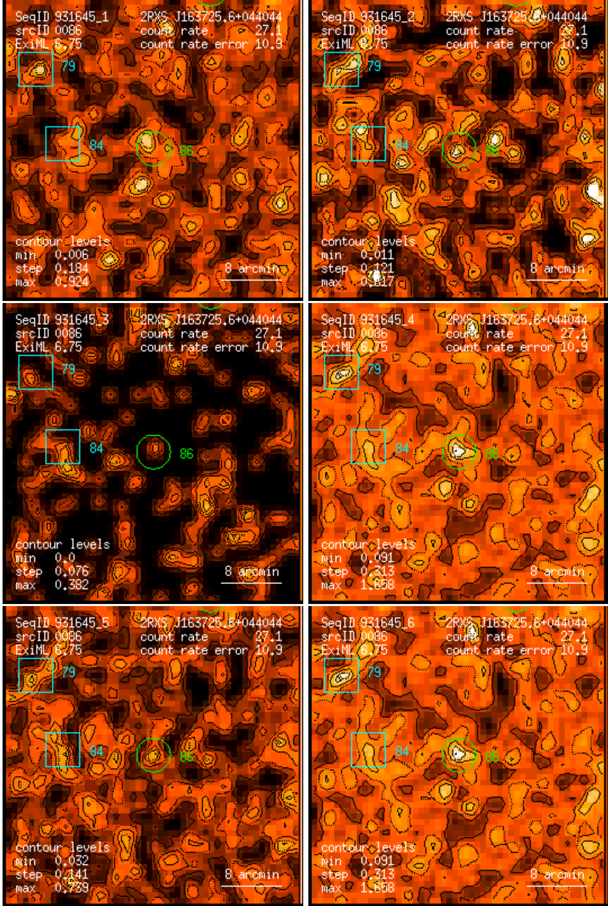
Figure 86: RASS 931645: detection 0086: band rate images, Gaussian filter: (1) PSPC channels 11 – 41, (2) 52 – 90, (3) 91 – 201, (4) 11 – 235, (5) 52 – 201, (6) 11 – 201. Broad band rates in counts/ks. Band rate contour levels in counts/ks/arcmin 2 .
