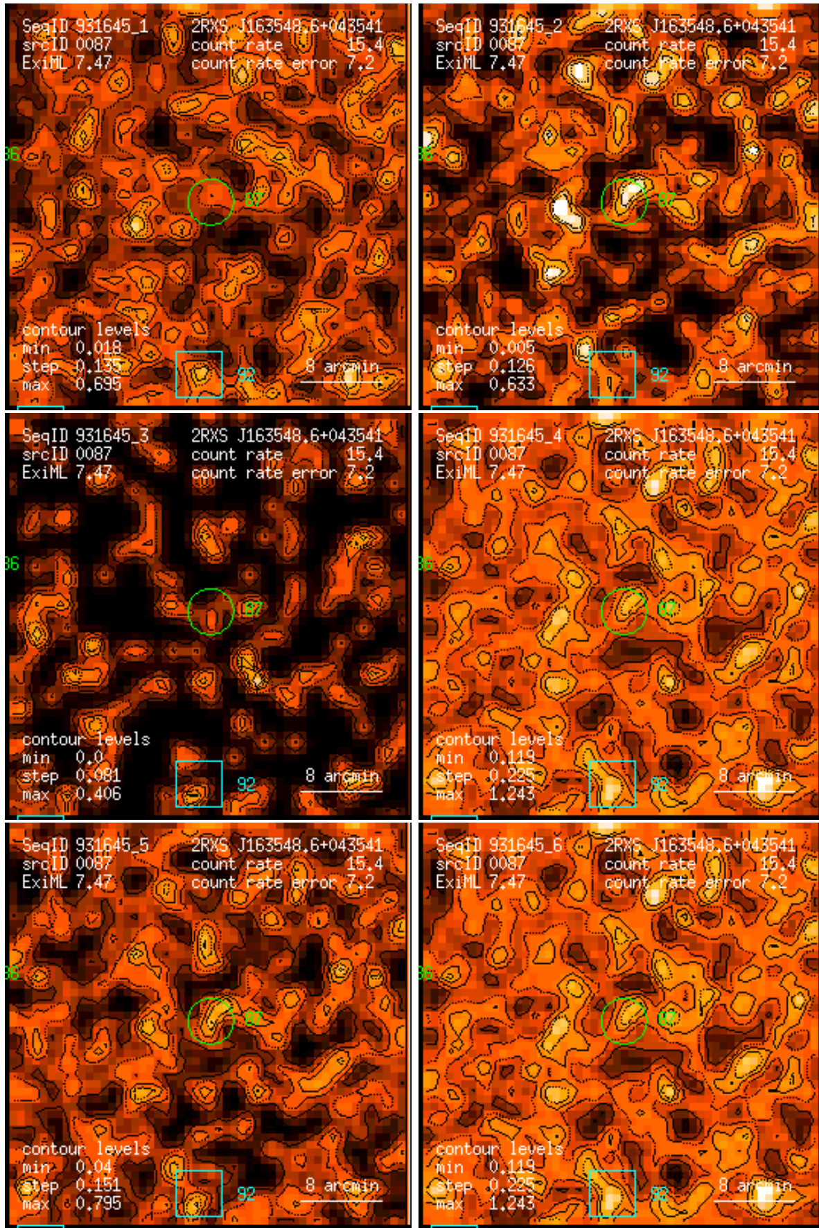
Figure 87: RASS 931645: detection 0087: band rate images, Gaussian filter: (1) PSPC channels 11 – 41, (2) 52 – 90, (3) 91 – 201, (4) 11 – 235, (5) 52 – 201, (6) 11 – 201. Broad band rates in counts/ks. Band rate contour levels in counts/ks/arcmin 2 .
