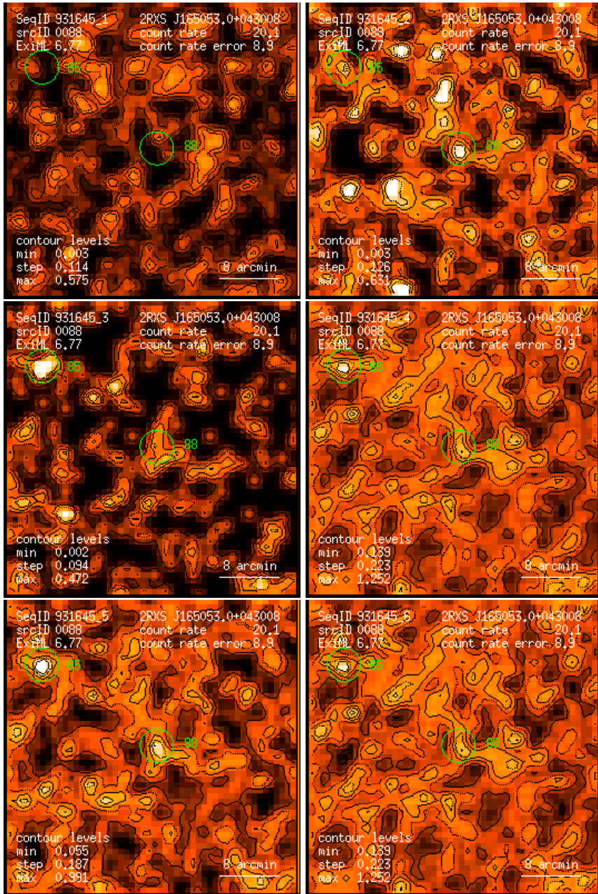
Figure 88: RASS 931645: detection 0088: band rate images, Gaussian filter: (1) PSPC channels 11 – 41, (2) 52 – 90, (3) 91 – 201, (4) 11 – 235, (5) 52 – 201, (6) 11 – 201. Broad band rates in counts/ks. Band rate contour levels in counts/ks/arcmin 2 .
