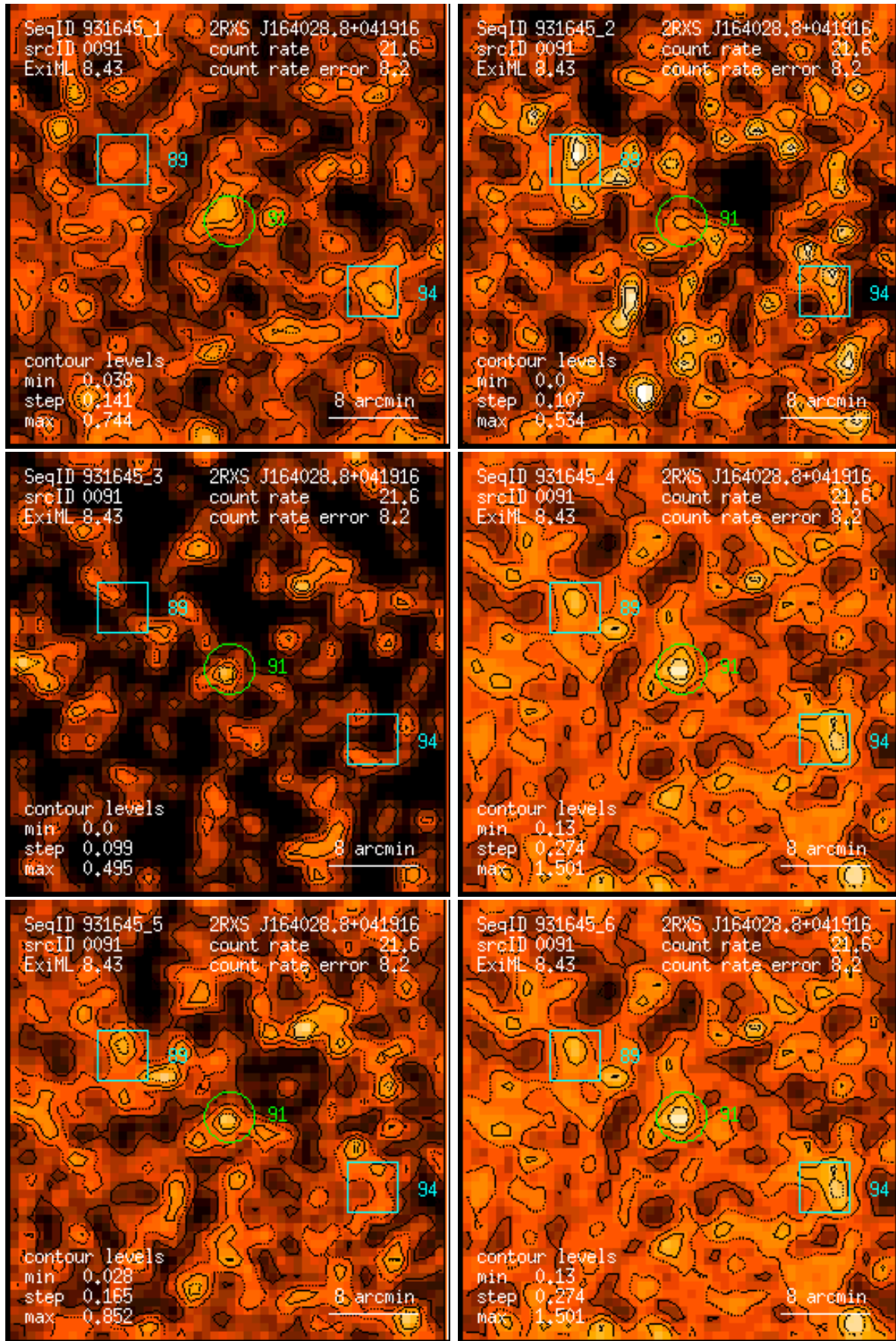
Figure 91: RASS 931645: detection 0091: band rate images, Gaussian filter: (1) PSPC channels 11 – 41, (2) 52 – 90, (3) 91 – 201, (4) 11 – 235, (5) 52 – 201, (6) 11 – 201. Broad band rates in counts/ks. Band rate contour levels in counts/ks/arcmin 2 .
