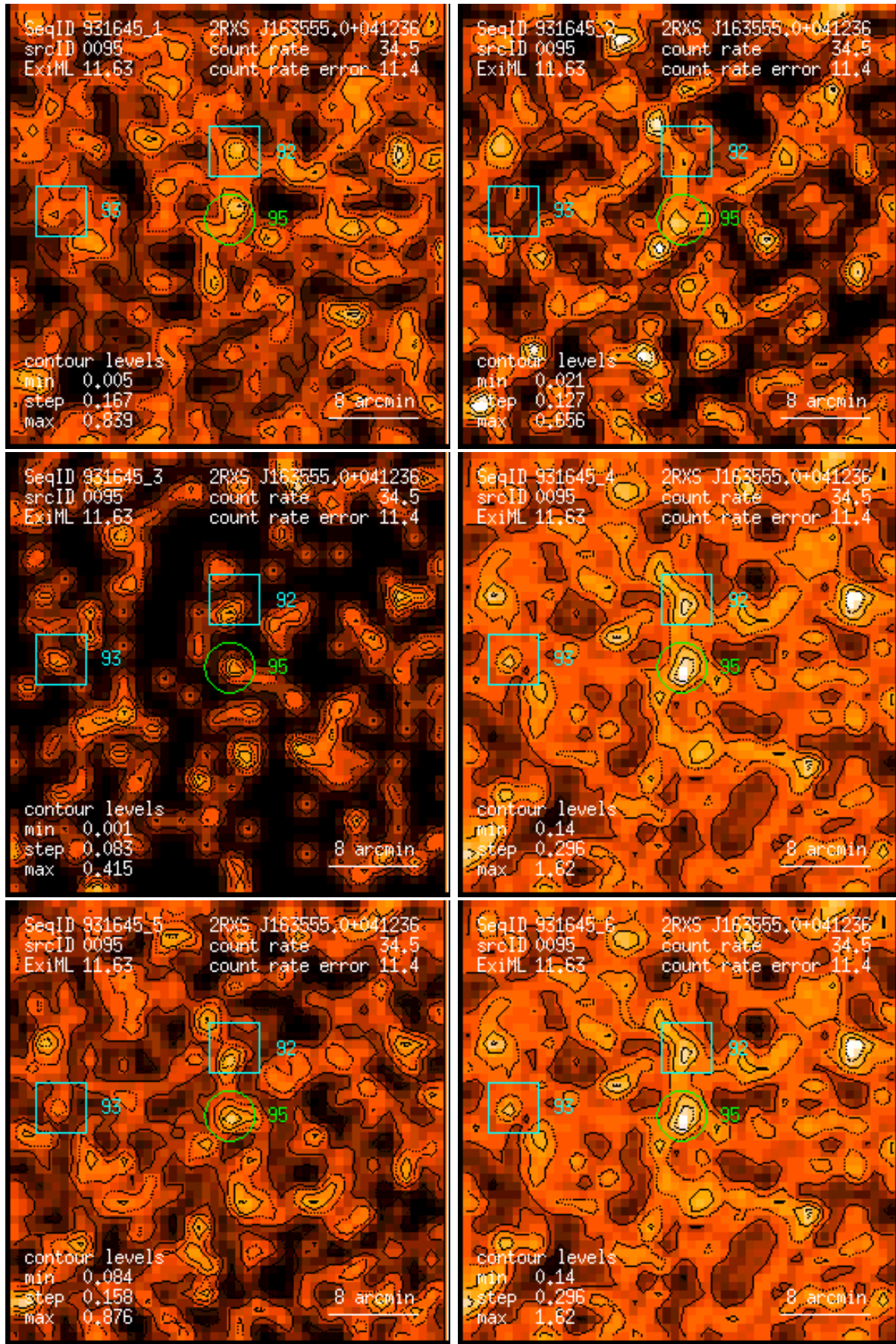
Figure 95: RASS 931645: detection 0095: band rate images, Gaussian filter: (1) PSPC channels 11 – 41, (2) 52 – 90, (3) 91 – 201, (4) 11 – 235, (5) 52 – 201, (6) 11 – 201. Broad band rates in counts/ks. Band rate contour levels in counts/ks/arcmin 2 .
