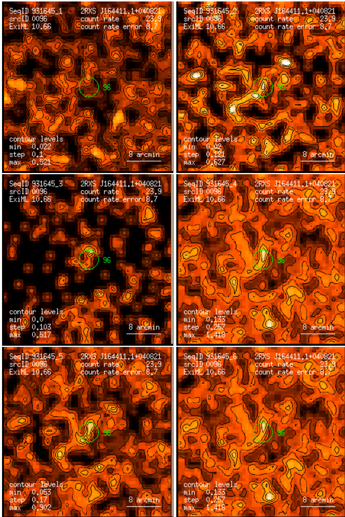
Figure 96: RASS 931645: detection 0096: band rate images, Gaussian filter: (1) PSPC channels 11 – 41, (2) 52 – 90, (3) 91 – 201, (4) 11 – 235, (5) 52 – 201, (6) 11 – 201. Broad band rates in counts/ks. Band rate contour levels in counts/ks/arcmin 2 .
