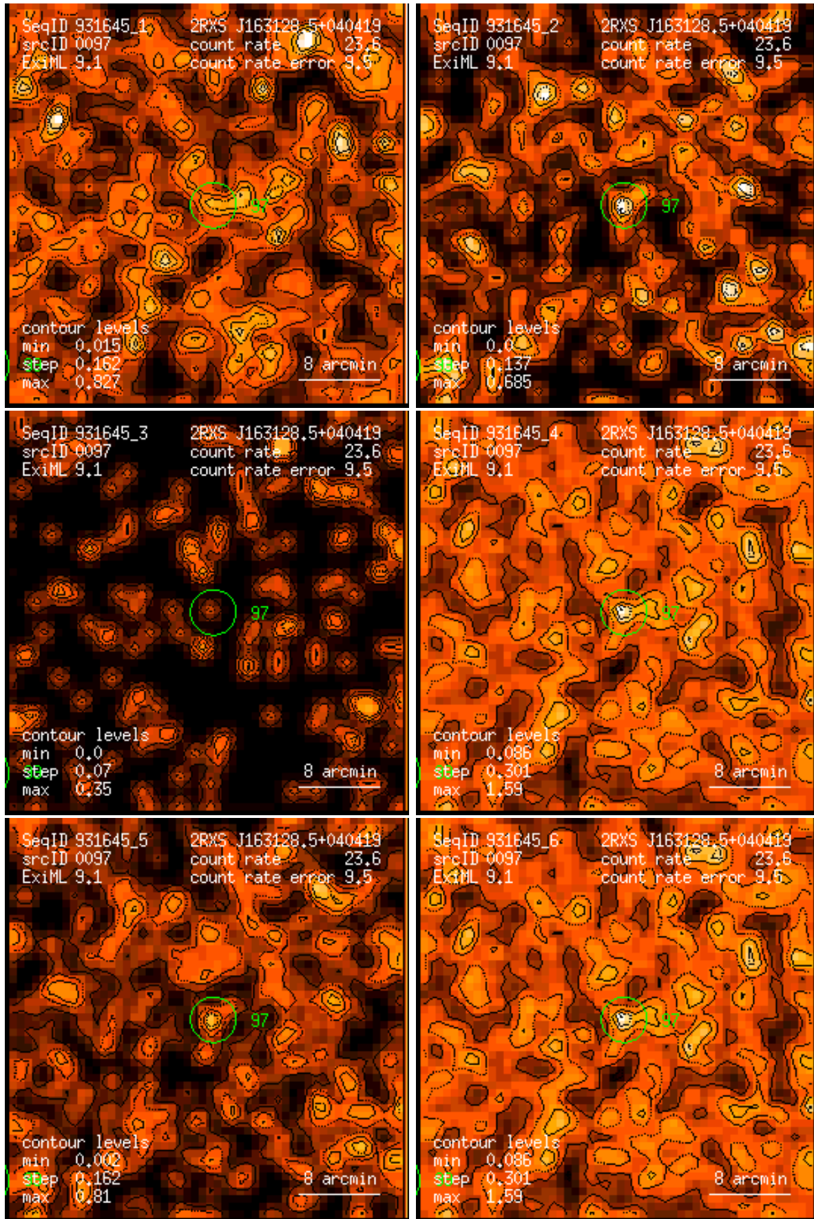
Figure 97: RASS 931645: detection 0097: band rate images, Gaussian filter: (1) PSPC channels 11 – 41, (2) 52 – 90, (3) 91 – 201, (4) 11 – 235, (5) 52 – 201, (6) 11 – 201. Broad band rates in counts/ks. Band rate contour levels in counts/ks/arcmin 2 .
