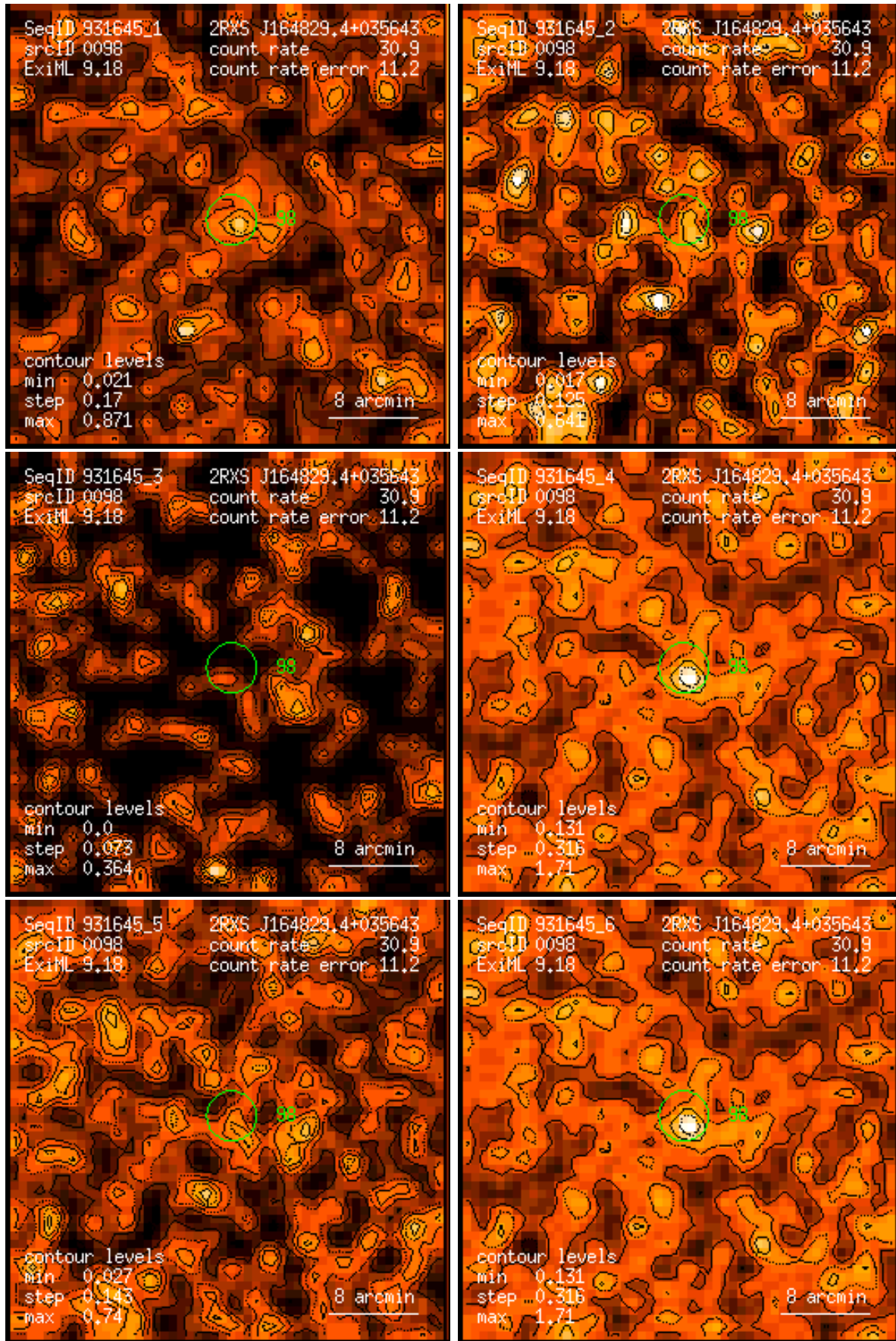
Figure 98: RASS 931645: detection 0098: band rate images, Gaussian filter: (1) PSPC channels 11 – 41, (2) 52 – 90, (3) 91 – 201, (4) 11 – 235, (5) 52 – 201, (6) 11 – 201. Broad band rates in counts/ks. Band rate contour levels in counts/ks/arcmin 2 .
