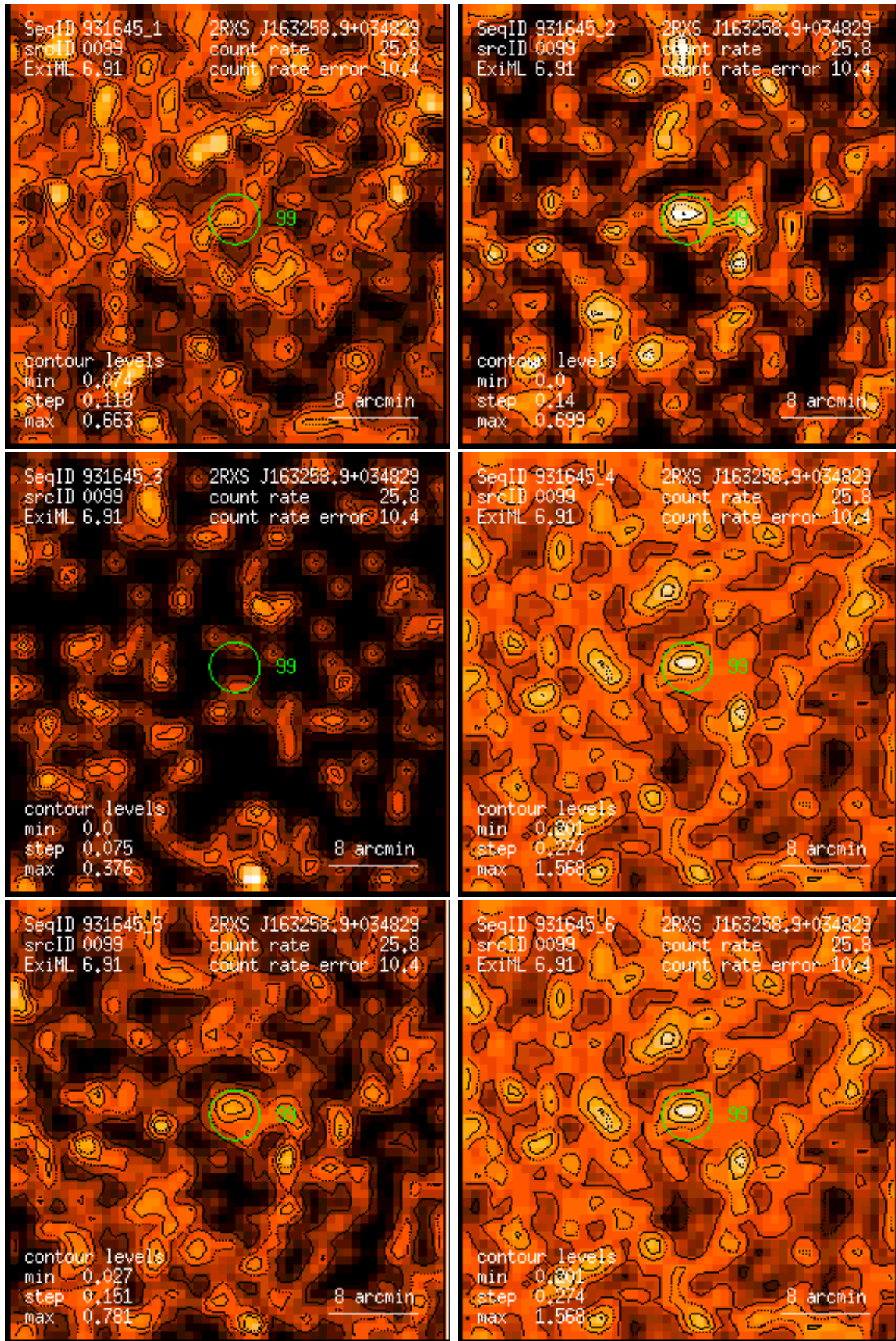
Figure 99: RASS 931645: detection 0099: band rate images, Gaussian filter: (1) PSPC channels 11 – 41, (2) 52 – 90, (3) 91 – 201, (4) 11 – 235, (5) 52 – 201, (6) 11 – 201. Broad band rates in counts/ks. Band rate contour levels in counts/ks/arcmin 2 .
