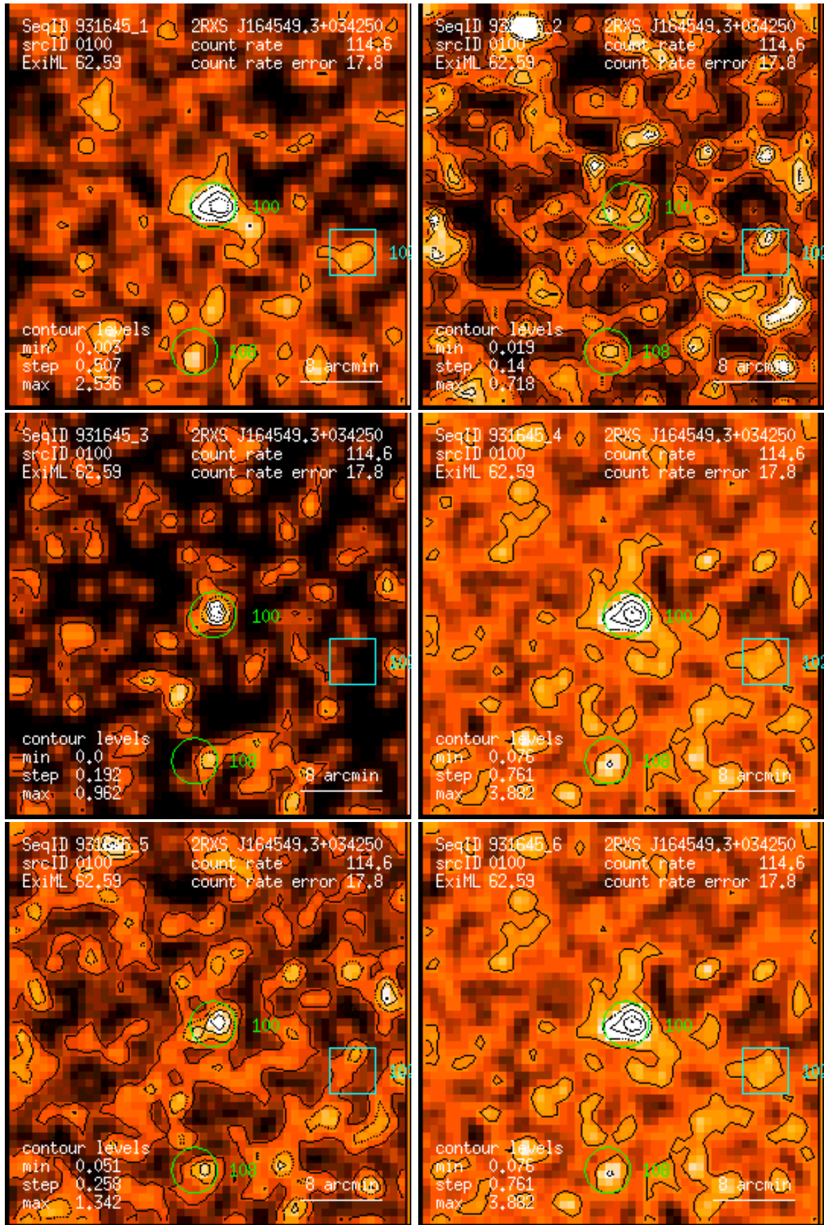
Figure 100: RASS 931645: detection 0100: band rate images, Gaussian filter: (1) PSPC channels 11 – 41, (2) 52 – 90, (3) 91 – 201, (4) 11 – 235, (5) 52 – 201, (6) 11 – 201. Broad band rates in counts/ks. Band rate contour levels in counts/ks/arcmin 2 .
