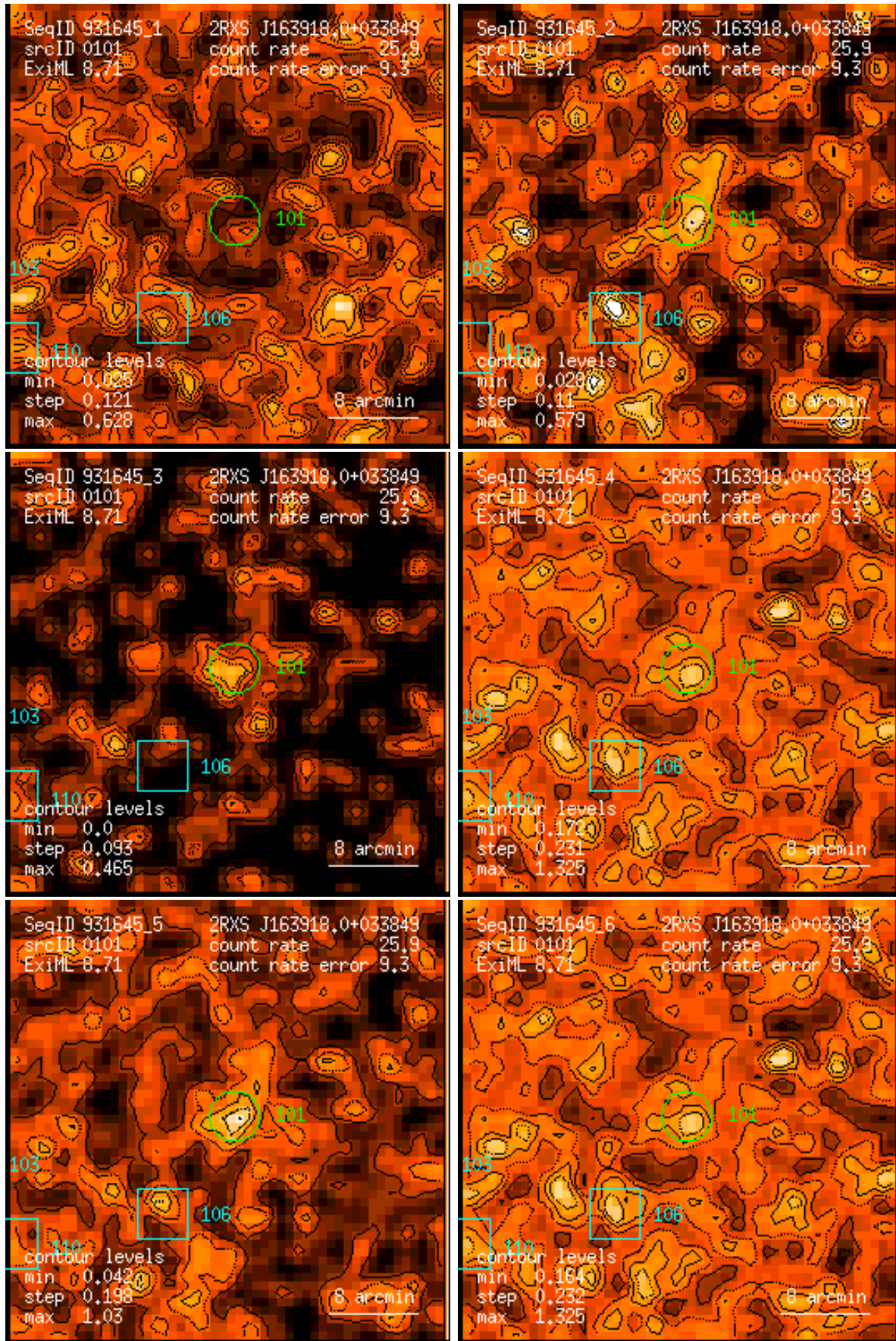
Figure 101: RASS 931645: detection 0101: band rate images, Gaussian filter: (1) PSPC channels 11 – 41, (2) 52 – 90, (3) 91 – 201, (4) 11 – 235, (5) 52 – 201, (6) 11 – 201. Broad band rates in counts/ks. Band rate contour levels in counts/ks/arcmin 2 .
