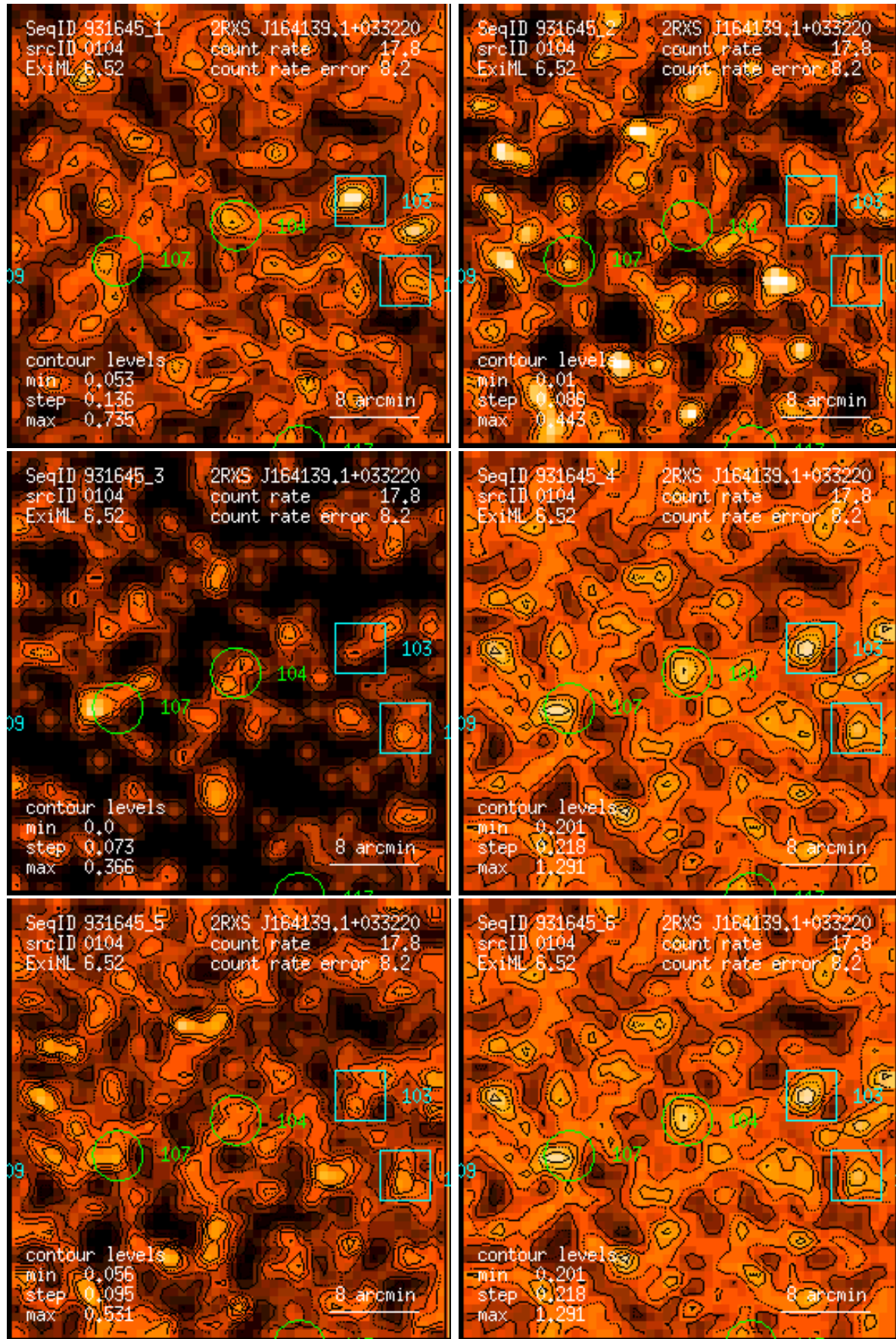
Figure 104: RASS 931645: detection 0104: band rate images, Gaussian filter: (1) PSPC channels 11 – 41, (2) 52 – 90, (3) 91 – 201, (4) 11 – 235, (5) 52 – 201, (6) 11 – 201. Broad band rates in counts/ks. Band rate contour levels in counts/ks/arcmin 2 .
