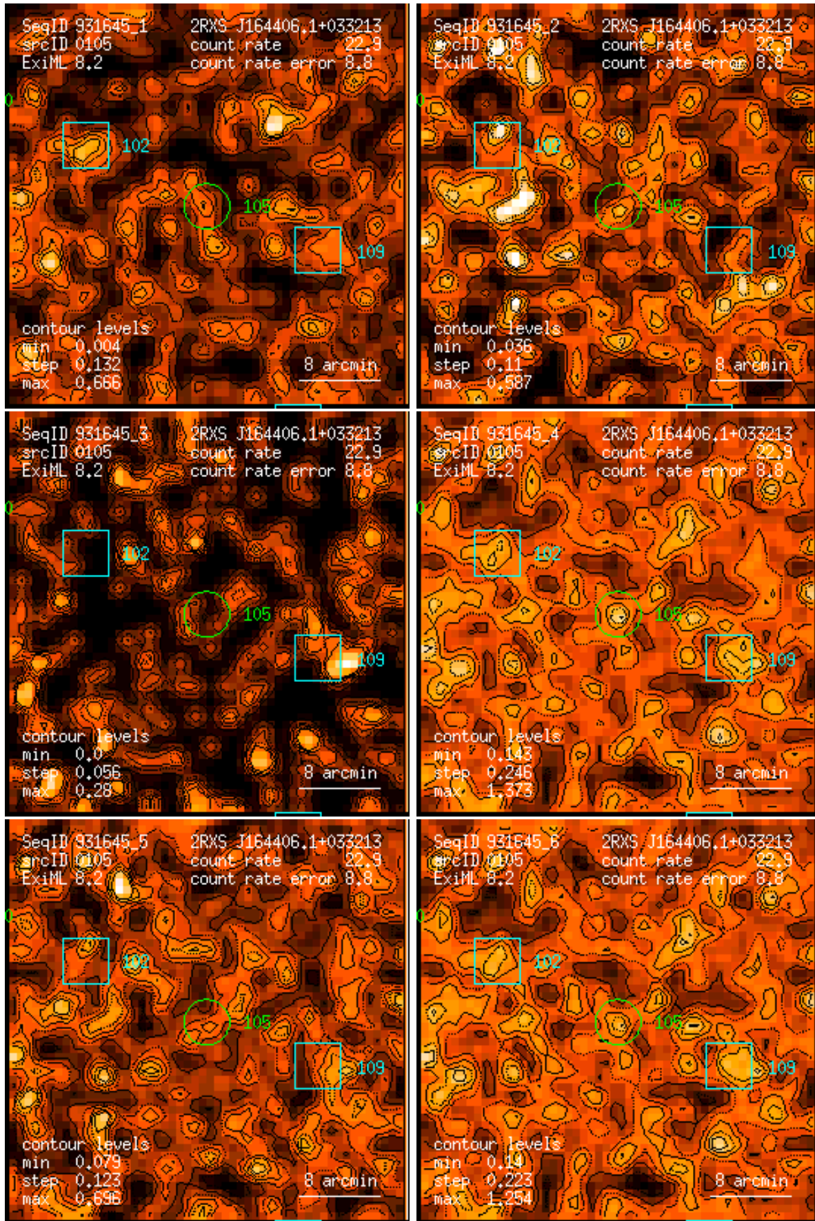
Figure 105: RASS 931645: detection 0105: band rate images, Gaussian filter: (1) PSPC channels 11 – 41, (2) 52 – 90, (3) 91 – 201, (4) 11 – 235, (5) 52 – 201, (6) 11 – 201. Broad band rates in counts/ks. Band rate contour levels in counts/ks/arcmin 2 .
