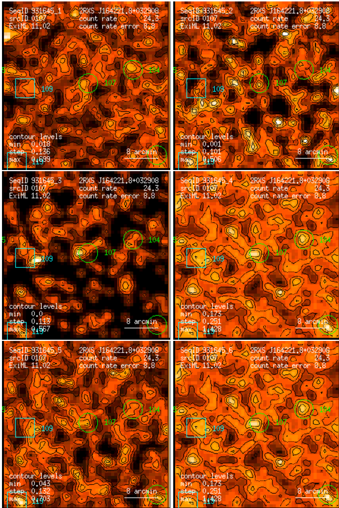
Figure 107: RASS 931645: detection 0107: band rate images, Gaussian filter: (1) PSPC channels 11 – 41, (2) 52 – 90, (3) 91 – 201, (4) 11 – 235, (5) 52 – 201, (6) 11 – 201. Broad band rates in counts/ks. Band rate contour levels in counts/ks/arcmin 2 .
