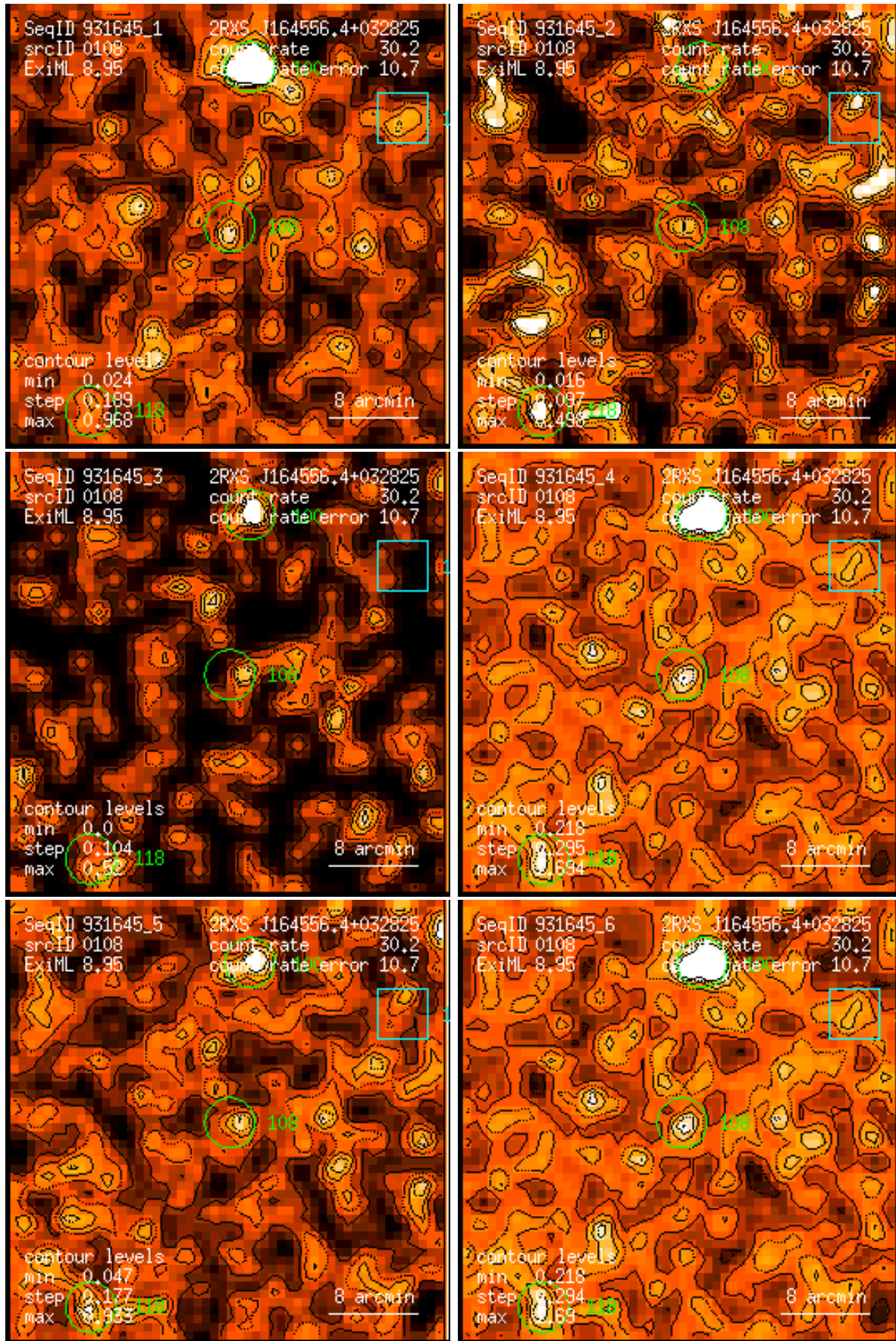
Figure 108: RASS 931645: detection 0108: band rate images, Gaussian filter: (1) PSPC channels 11 – 41, (2) 52 – 90, (3) 91 – 201, (4) 11 – 235, (5) 52 – 201, (6) 11 – 201. Broad band rates in counts/ks. Band rate contour levels in counts/ks/arcmin 2 .
