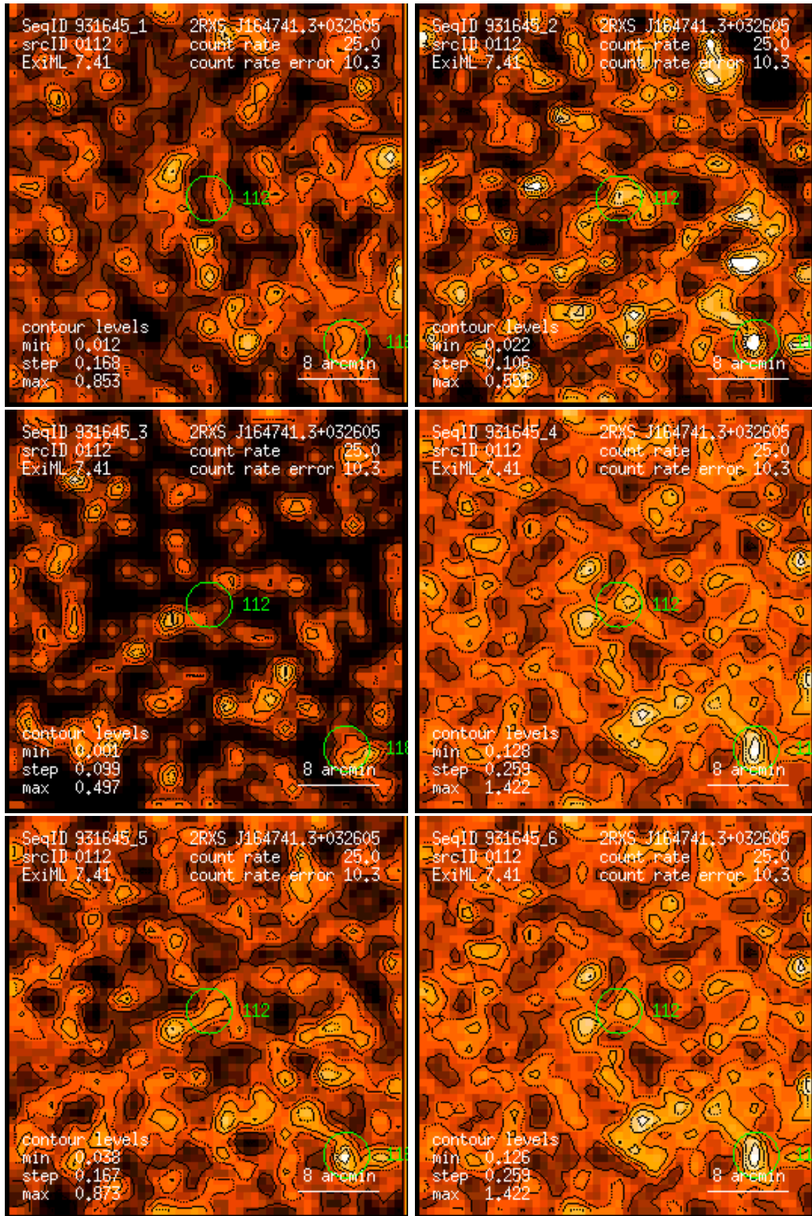
Figure 112: RASS 931645: detection 0112: band rate images, Gaussian filter: (1) PSPC channels 11 – 41, (2) 52 – 90, (3) 91 – 201, (4) 11 – 235, (5) 52 – 201, (6) 11 – 201. Broad band rates in counts/ks. Band rate contour levels in counts/ks/arcmin 2 .
