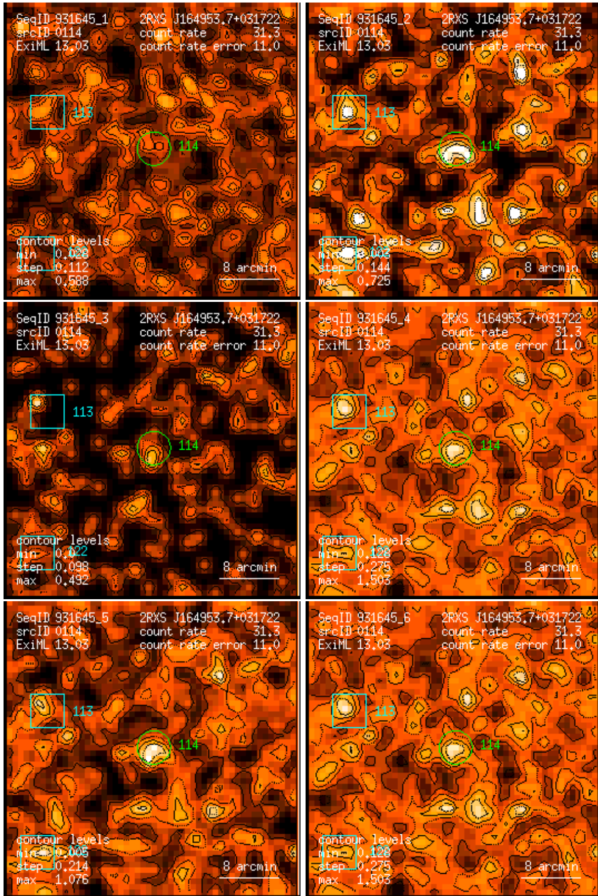
Figure 114: RASS 931645: detection 0114: band rate images, Gaussian filter: (1) PSPC channels 11 – 41, (2) 52 – 90, (3) 91 – 201, (4) 11 – 235, (5) 52 – 201, (6) 11 – 201. Broad band rates in counts/ks. Band rate contour levels in counts/ks/arcmin 2 .
