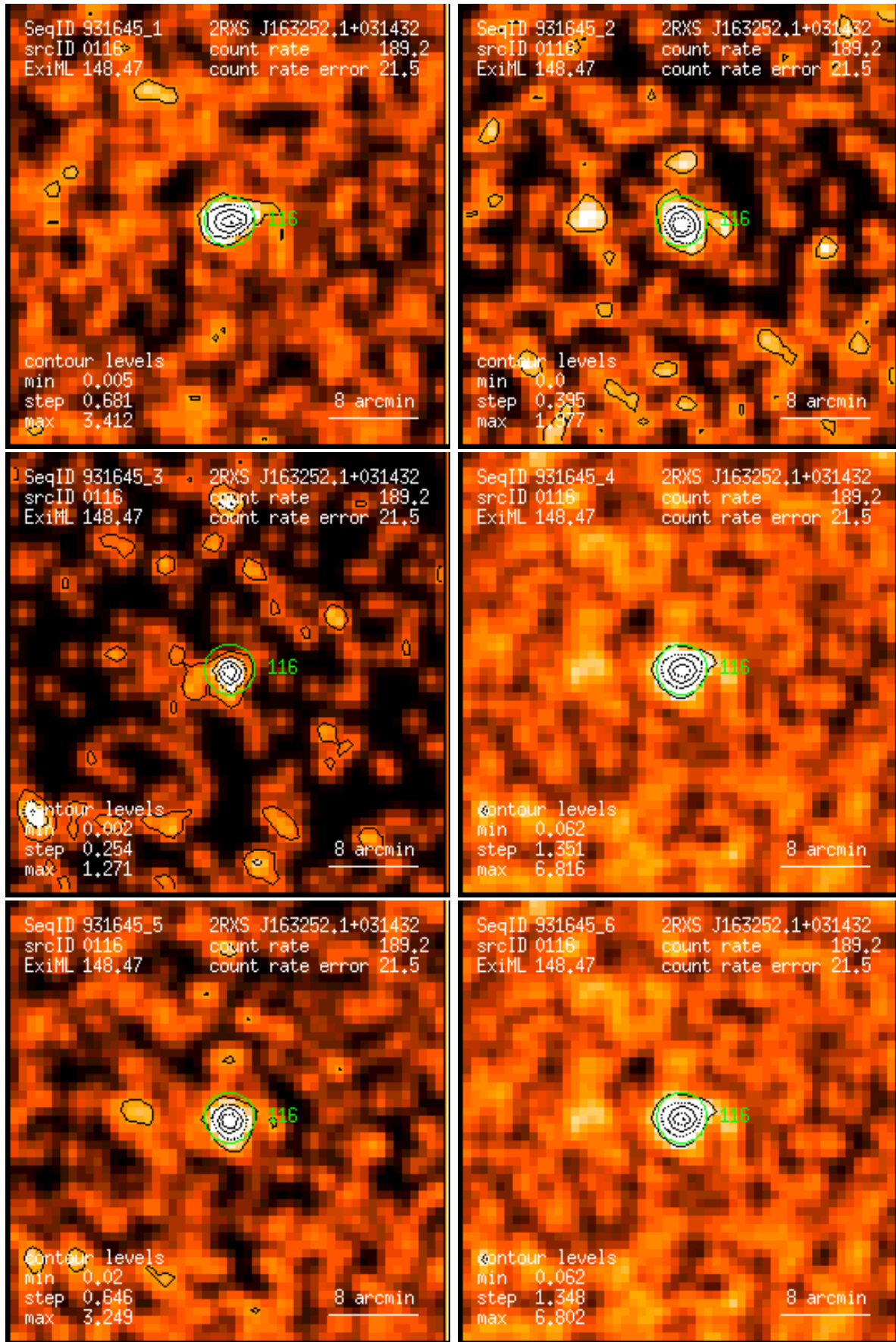
Figure 116: RASS 931645: detection 0116: band rate images, Gaussian filter: (1) PSPC channels 11 – 41, (2) 52 – 90, (3) 91 – 201, (4) 11 – 235, (5) 52 – 201, (6) 11 – 201. Broad band rates in counts/ks. Band rate contour levels in counts/ks/arcmin 2 .
