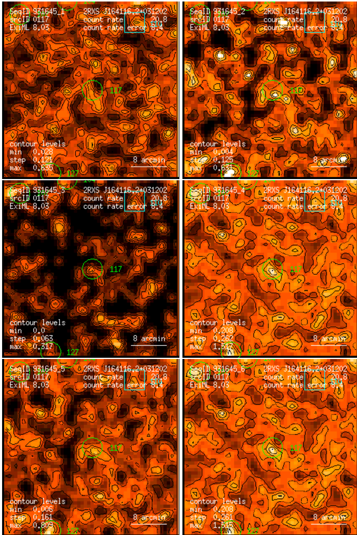
Figure 117: RASS 931645: detection 0117: band rate images, Gaussian filter: (1) PSPC channels 11 – 41, (2) 52 – 90, (3) 91 – 201, (4) 11 – 235, (5) 52 – 201, (6) 11 – 201. Broad band rates in counts/ks. Band rate contour levels in counts/ks/arcmin 2 .
