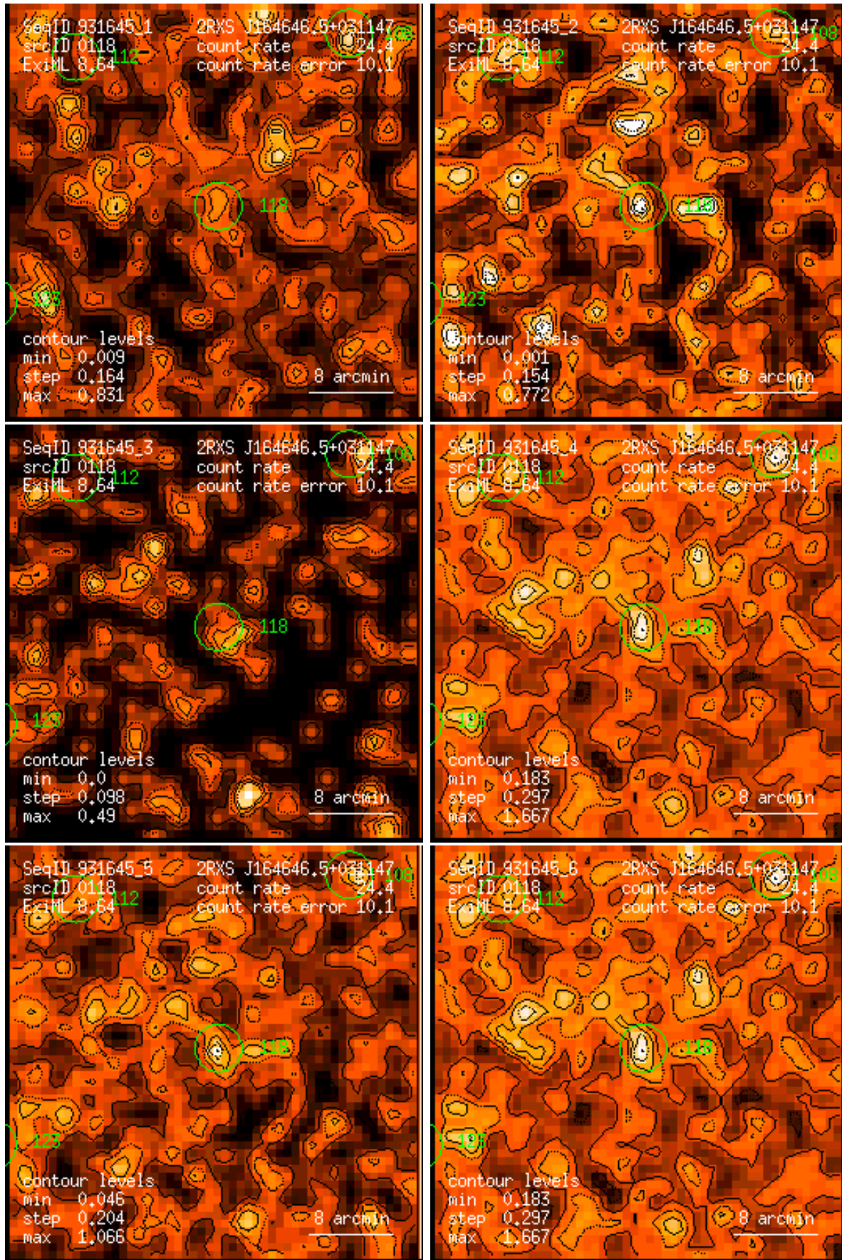
Figure 118: RASS 931645: detection 0118: band rate images, Gaussian filter: (1) PSPC channels 11 – 41, (2) 52 – 90, (3) 91 – 201, (4) 11 – 235, (5) 52 – 201, (6) 11 – 201. Broad band rates in counts/ks. Band rate contour levels in counts/ks/arcmin 2 .
