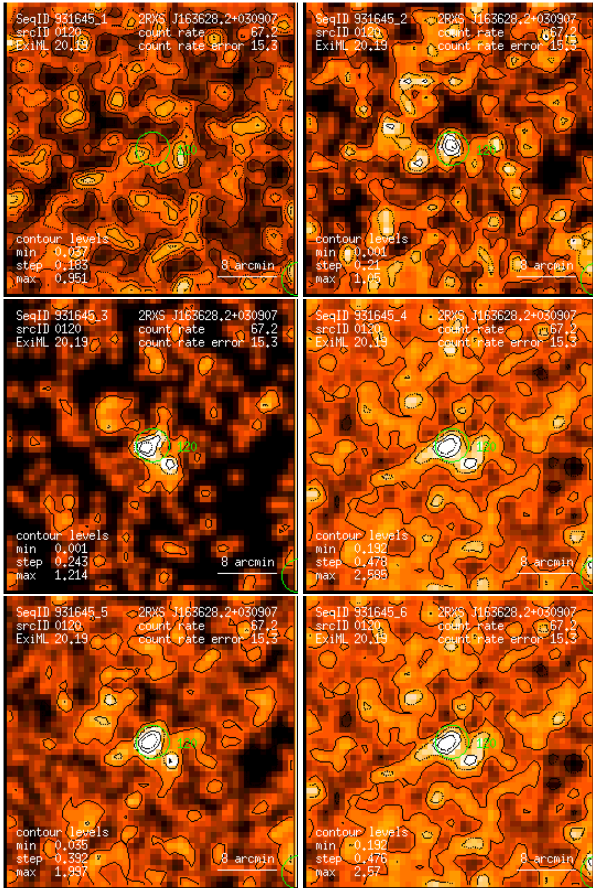
Figure 120: RASS 931645: detection 0120: band rate images, Gaussian filter: (1) PSPC channels 11 – 41, (2) 52 – 90, (3) 91 – 201, (4) 11 – 235, (5) 52 – 201, (6) 11 – 201. Broad band rates in counts/ks. Band rate contour levels in counts/ks/arcmin 2 .
