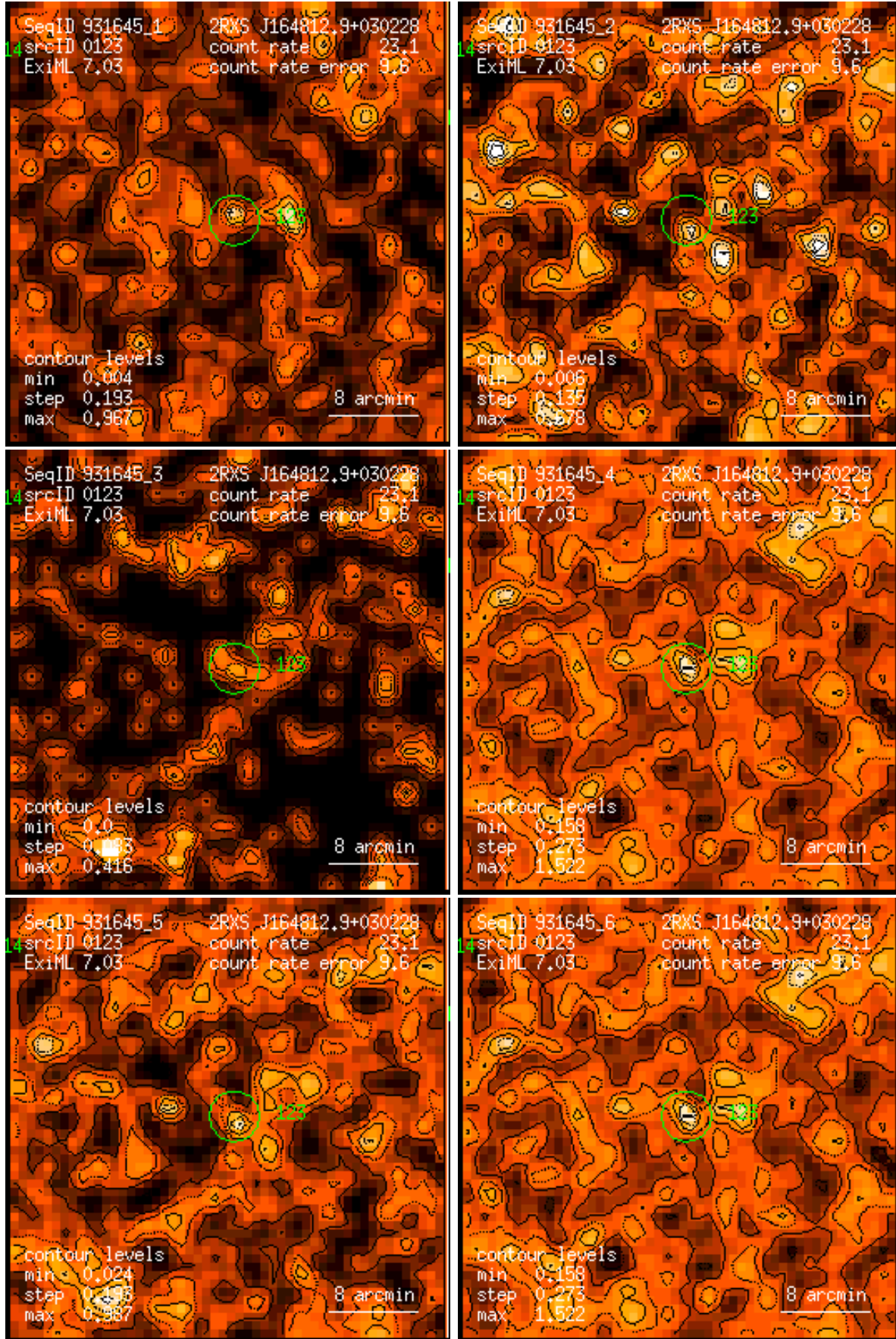
Figure 123: RASS 931645: detection 0123: band rate images, Gaussian filter: (1) PSPC channels 11 – 41, (2) 52 – 90, (3) 91 – 201, (4) 11 – 235, (5) 52 – 201, (6) 11 – 201. Broad band rates in counts/ks. Band rate contour levels in counts/ks/arcmin 2 .
