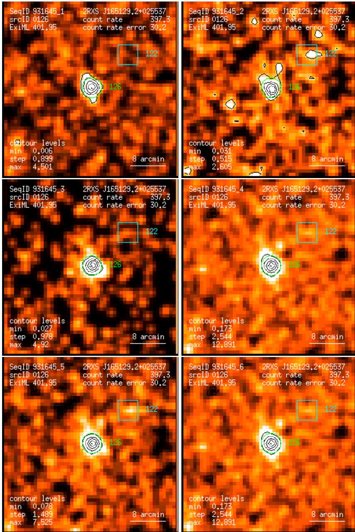
Figure 126: RASS 931645: detection 0126: band rate images, Gaussian filter: (1) PSPC channels 11 – 41, (2) 52 – 90, (3) 91 – 201, (4) 11 – 235, (5) 52 – 201, (6) 11 – 201. Broad band rates in counts/ks. Band rate contour levels in counts/ks/arcmin 2 .
