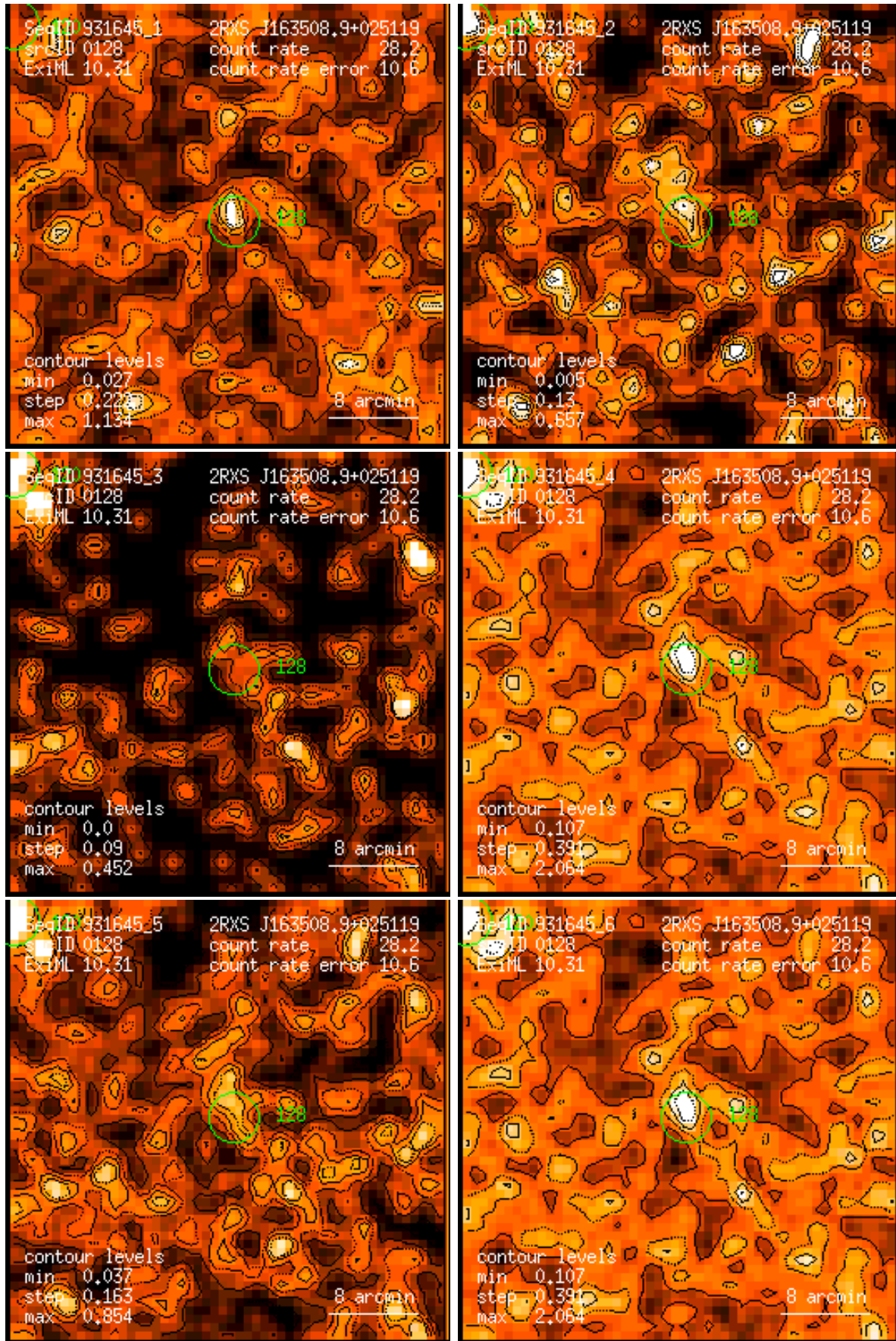
Figure 128: RASS 931645: detection 0128: band rate images, Gaussian filter: (1) PSPC channels 11 – 41, (2) 52 – 90, (3) 91 – 201, (4) 11 – 235, (5) 52 – 201, (6) 11 – 201. Broad band rates in counts/ks. Band rate contour levels in counts/ks/arcmin 2 .
