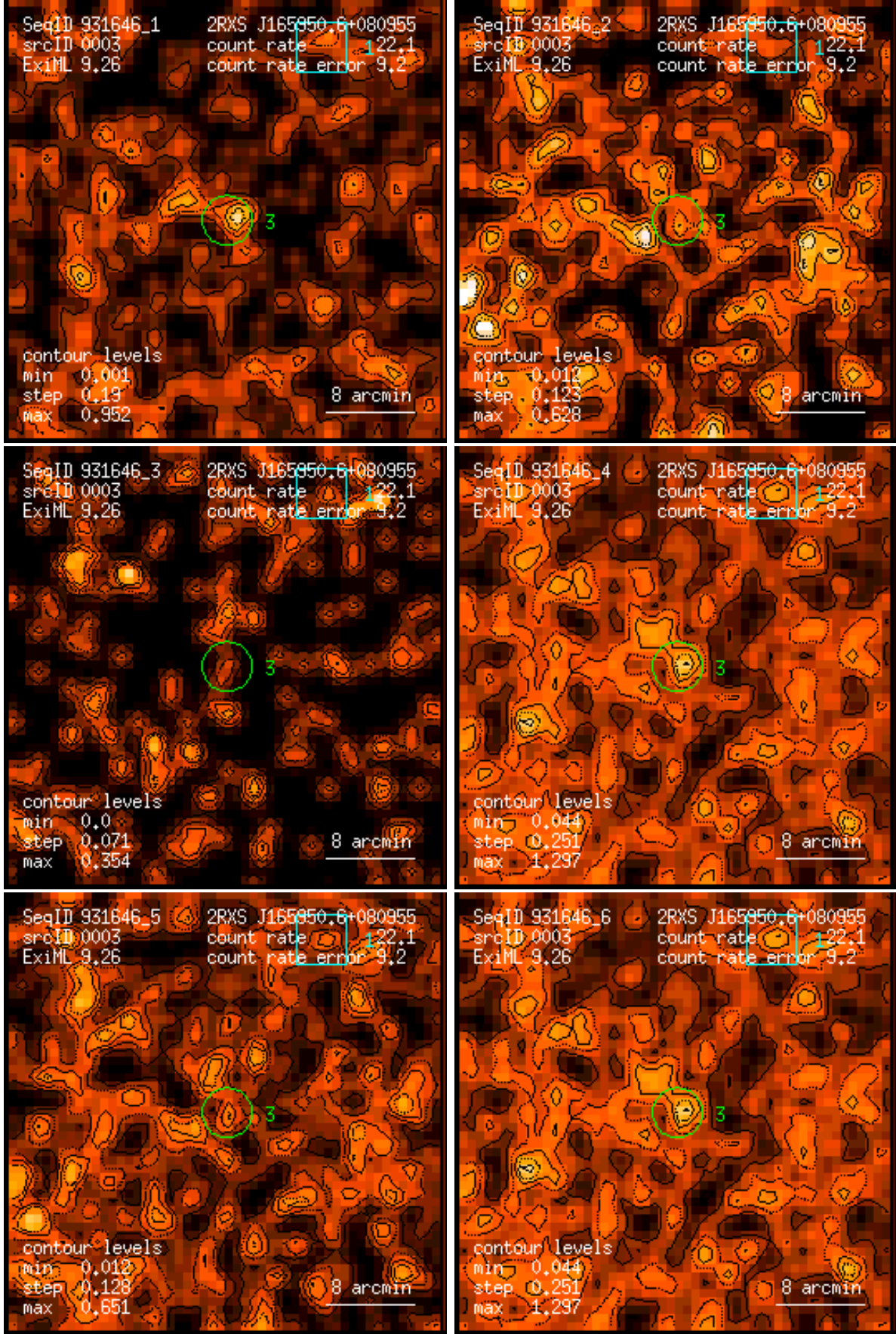
Figure 3: RASS 931646: detection 0003: band rate images, Gaussian filter: (1) PSPC channels 11 – 41, (2) 52 – 90, (3) 91 – 201, (4) 11 – 235, (5) 52 – 201, (6) 11 – 201. Broad band rates in counts/ks. Band rate contour levels in counts/ks/arcmin 2 .
