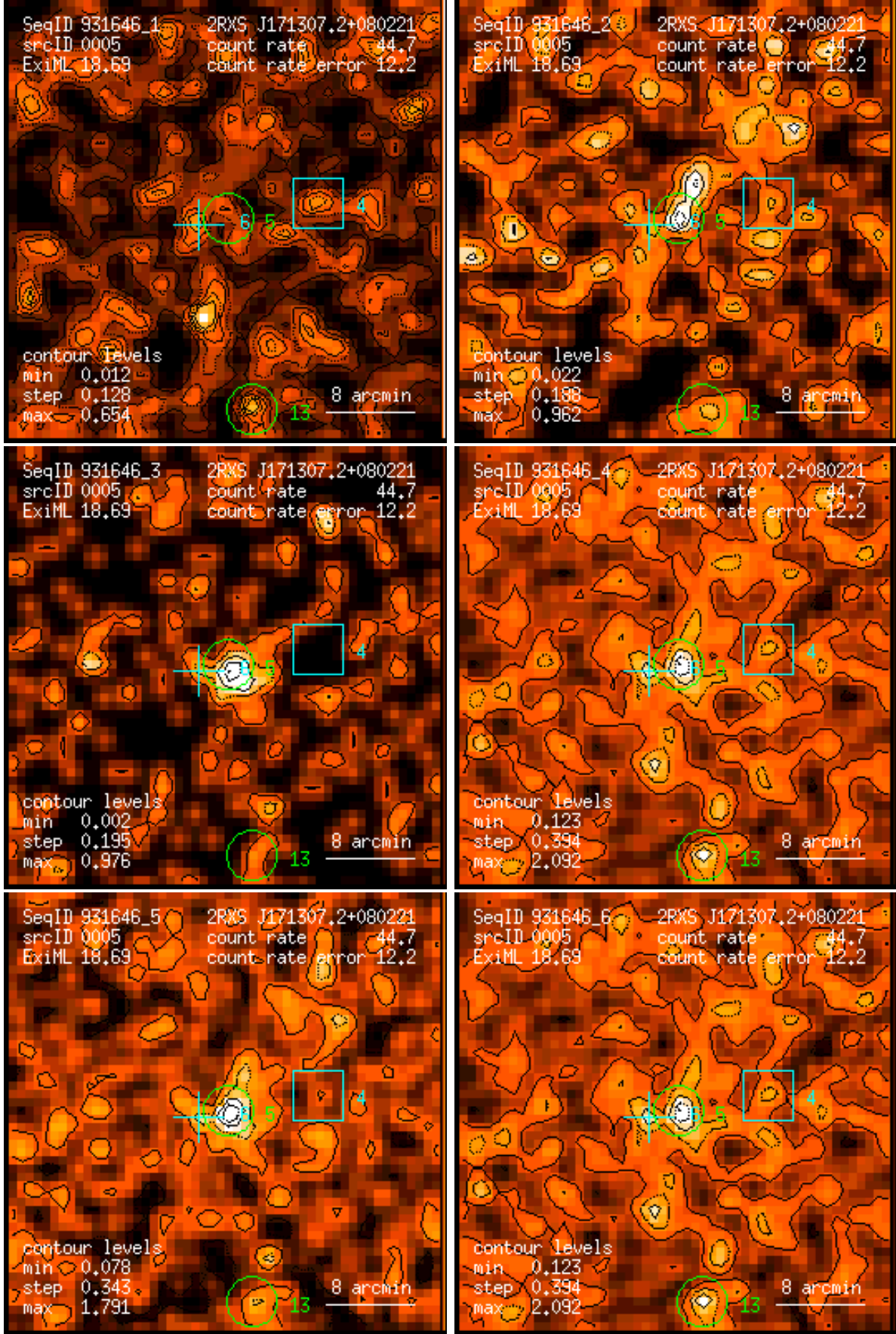
Figure 5: RASS 931646: detection 0005: band rate images, Gaussian filter: (1) PSPC channels 11 – 41, (2) 52 – 90, (3) 91 – 201, (4) 11 – 235, (5) 52 – 201, (6) 11 – 201. Broad band rates in counts/ks. Band rate contour levels in counts/ks/arcmin 2 .
