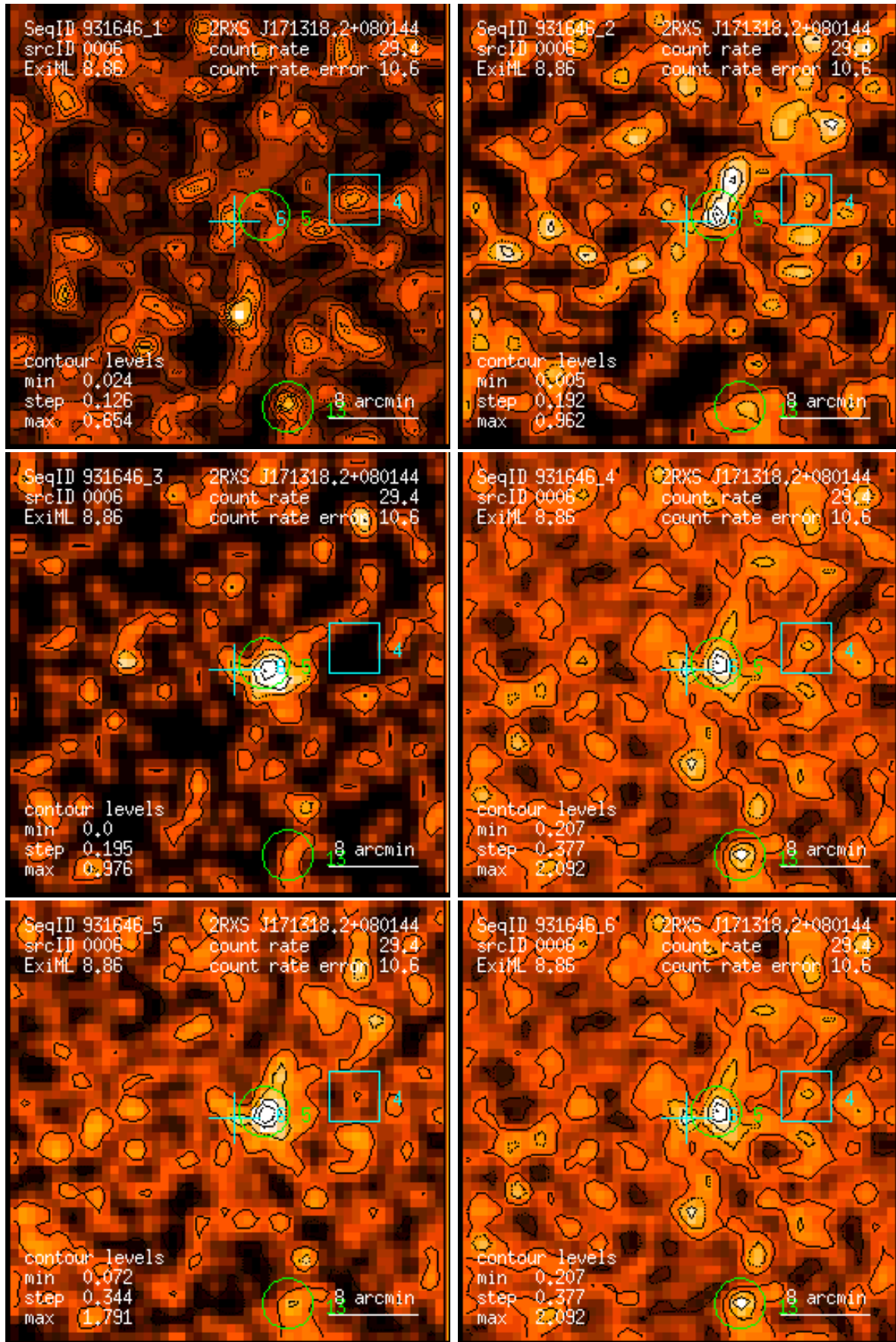
Figure 6: RASS 931646: detection 0006: band rate images, Gaussian filter: (1) PSPC channels 11 – 41, (2) 52 – 90, (3) 91 – 201, (4) 11 – 235, (5) 52 – 201, (6) 11 – 201. Broad band rates in counts/ks. Band rate contour levels in counts/ks/arcmin 2 .
