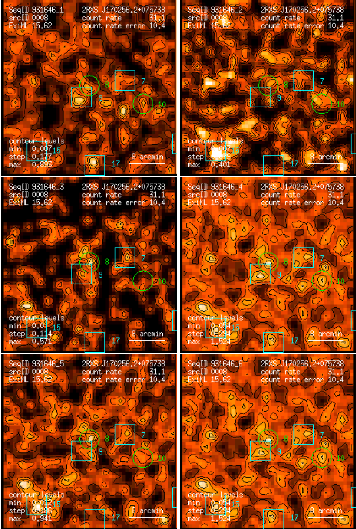
Figure 8: RASS 931646: detection 0008: band rate images, Gaussian filter: (1) PSPC channels 11 – 41, (2) 52 – 90, (3) 91 – 201, (4) 11 – 235, (5) 52 – 201, (6) 11 – 201. Broad band rates in counts/ks. Band rate contour levels in counts/ks/arcmin 2 .
