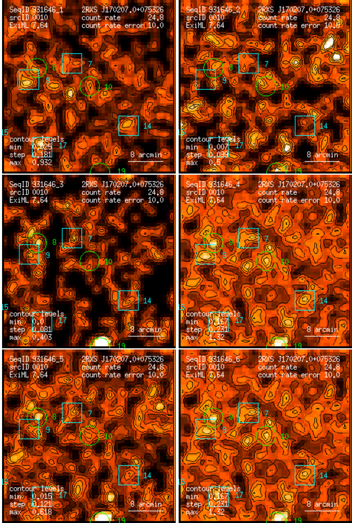
Figure 10: RASS 931646: detection 0010: band rate images, Gaussian filter: (1) PSPC channels 11 – 41, (2) 52 – 90, (3) 91 – 201, (4) 11 – 235, (5) 52 – 201, (6) 11 – 201. Broad band rates in counts/ks. Band rate contour levels in counts/ks/arcmin 2 .
